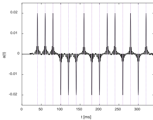
Fig. 4. Echo signal after correlation with elementary FFM signals and subtraction.
