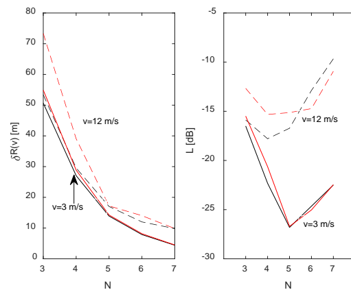
Fig. 19. Resolution and level of side lobes (marked as in Fig. 18).
