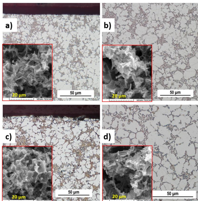
Fig. 5. Microstructure of casting A75 and A90 (OM – etc. Dix-Keller, SEM – etc. HCl); (a) surface area A75; (b) central region A75; c) surface area A90; (d) central region A90
