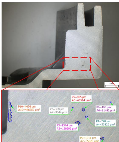
Fig. 3. Methodology of measuring areal porosity on control sections
