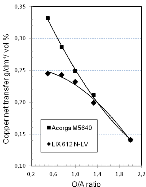
Fig. 7. Copper net transfer in organic phase at 30 vol % of reagent as a function of overall extraction O/A ratio, raffinate, pH 0.75
