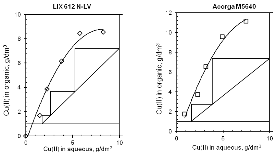
Fig. 5. The McCabe-Thiele diagram for 30vol% of LIX 612 N-LV and Acorga M5640 in Escald 100, feed: raffinate I, pH 0.75, O/A 1.33
