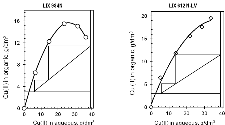
Fig. 1. The McCabe-Thiele diagram for 30 vol% of LIX 984 N and LIX 612 N-LV in Escaid 100, feed: PLS I, pH 2.2, O/A 4.0
