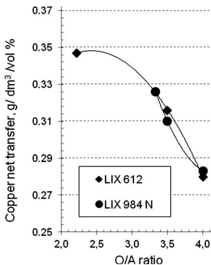
Fig. 2. Copper net transfer in organic phase at 30 vol % of reagent as a function of overall extraction O/A ratio, PLS I
