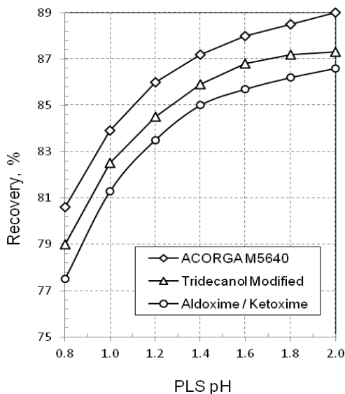
Fig. 6. SX circuit recovery comparison (30 vol % extractant, 25 g/dm 3 of copper in PLS) (Moore et al., 1999)
