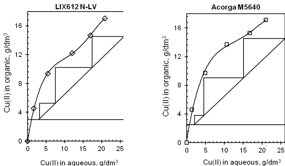
Fig. 3. The McCabe–Thiele diagram for 30 vol% of LIX 612 N-LV and Acorga M5640 in Escaid 100, feed: PLS II, pH 2.0, O/A 2.0
