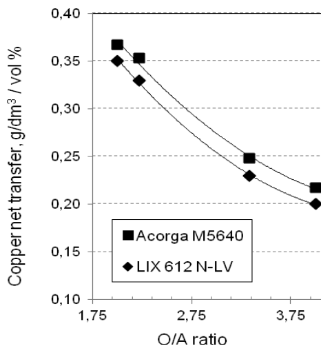
Fig. 4. Copper net transfer in organic at 30 vol % of reagent as a function of overall extraction O/A ratio, PLS II
