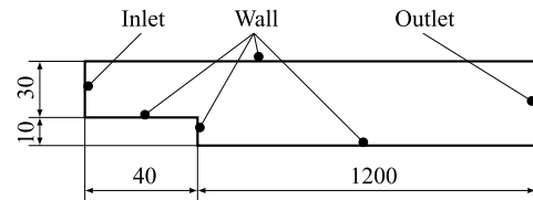
Fig. 16. Geometric model of backward-facing step (dimensions in mm).
