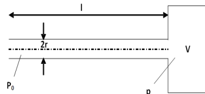
Fig. 1. Pressure chamber with inlet pipe: r, l - tube dimensions, P_0 - input pressure (force), P - pressure in transducer chamber
