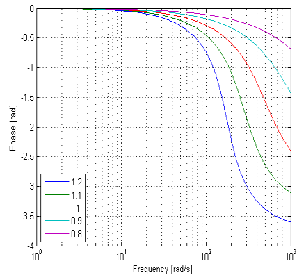
Fig. 5. Logarithmic phase response of a pneumatic transducer described by means of differential equation with fractional derivatives of non-integer orders in the range (0.8-1.2)
