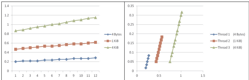
Fig. 8. Experimental results using the default allocator on VxWorks 6.7
