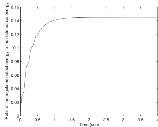
Fig. 5. Ratio of the regulated output energy to the disturbance noise energy, \left( \int_0^{T_f} z^T(t)z(t) dt / \int_0^{T_f} w^T(t)w(t) dt \right) .
