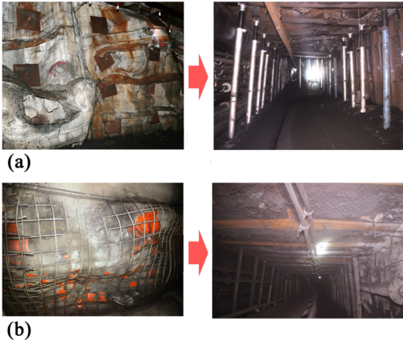
Fig. 11. Comparison of FFPC and RCPR: (a) Chengjiao mine and (b) Zhongxing mine
