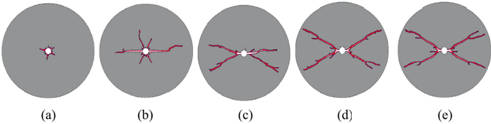
Fig. 3. Comparison of ordinary blasting and BCTE: (a) ordinary blasting (b) BCTE, \beta = 15^\circ , (c) BCTE, \beta = 25^\circ , (d) BCTE, \beta = 35^\circ , (e) BCTE, \beta = 45^\circ
