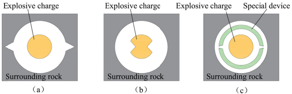
Fig. 1. Types of cumulative blasts: (a) notched blasting, (b) energy-concentrated charge blasting, (c) energy-collecting tube blasting
