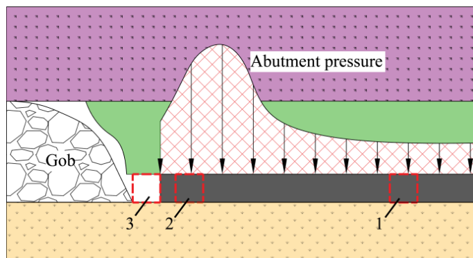
Fig. 7. Lateral abutment pressure and selection of roadway position
