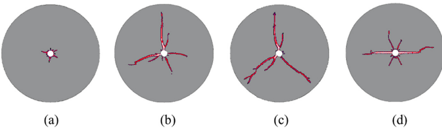
Fig. 4. Comparison of ordinary blasting and BCTE: (a) ordinary blasting (b) BCTE, \alpha = 90^\circ , (c) BCTE, \alpha = 120^\circ , (d) BCTE, \alpha = 180^\circ
