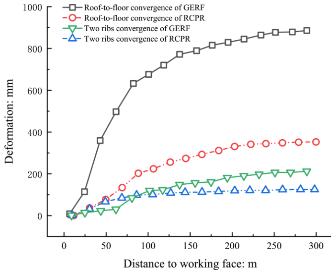
Fig. 12. Roof-to-floor convergence and the convergence of the two ribs in haulageway of Jinfeng mine
