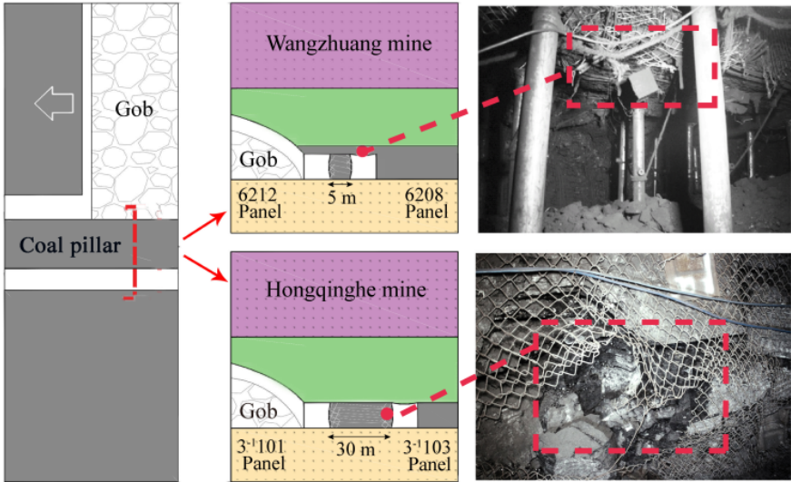
Fig. 9. Roadway damage before using BCTE
