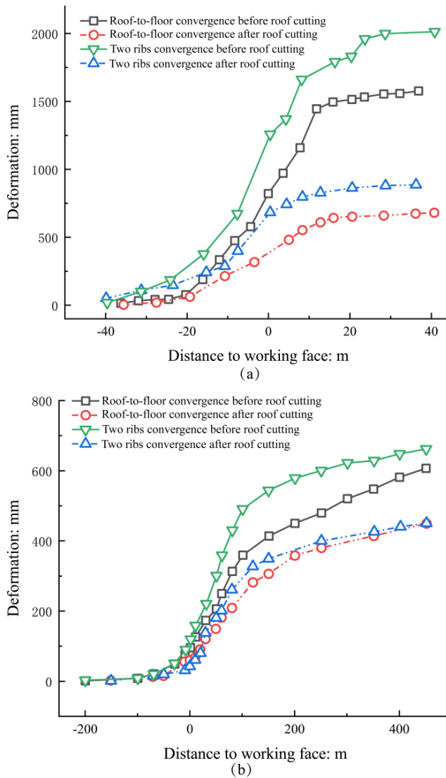
Fig. 10. Roof-to-floor convergence and convergence of the two ribs for tailgates: (a) Wangzhuang mine and (b) Hongqinghe mine
