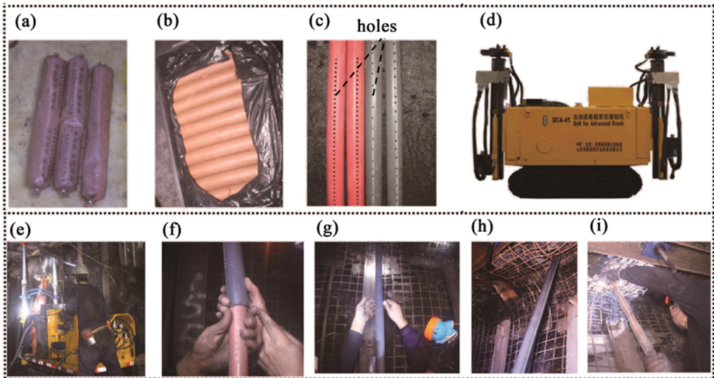
Fig. 6. Device, material, technological process of BCTE: (a) explosive cartridge, (b) stemming, (c) energy-collecting tube, (d) roof cutting machinery, (e) drill holes, (f) stuff the explosive cartridge into the energy-collecting tube, (g) fix the explosive cartridge, (h) insert explosive cartridge and energy-collecting tube into boreholes, (i) sealing boreholes with stemming
