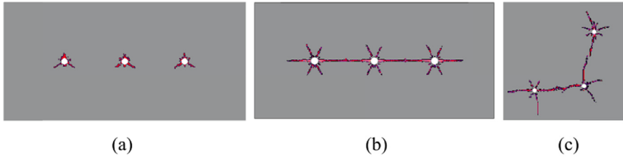
Fig. 5. Comparison of joint blasting: (a) ordinary blasting (b) BCTE, \alpha = 180^\circ , (c) BCTE, \alpha = 90^\circ
