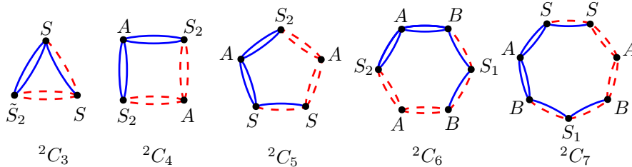
Fig. 2. A locally irregular coloring of the multicycles. The meaning of vertex labels will be explained in Theorem 2.3
