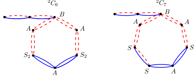
Fig. 5. The initial coloring of {}^2C_6 with spike and {}^2C_7 with spike
