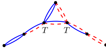
Fig. 10. The particular coloring of special pair T with spikes
