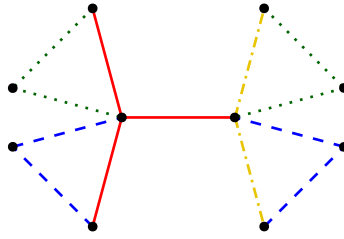
Fig. 1. The bow-tie graph B and its locally irregular coloring with four colors
