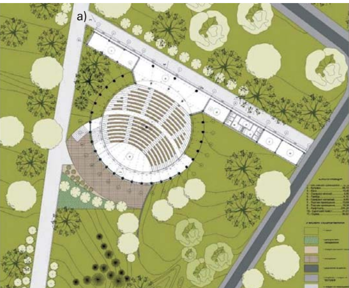
il. 8. Conceptual solution to “landscape” theatre in B.Khmelnytskyi Culture and Recreation Park in Lviv: a) scheme of outdoor theatre plan; b) project solution to “landscape” theatre construction (Authors: prof. V. Proskuryakov, s.lecturer Yu. Bohdanova, assist. I. Gumennyk, st. O. Olenych)
