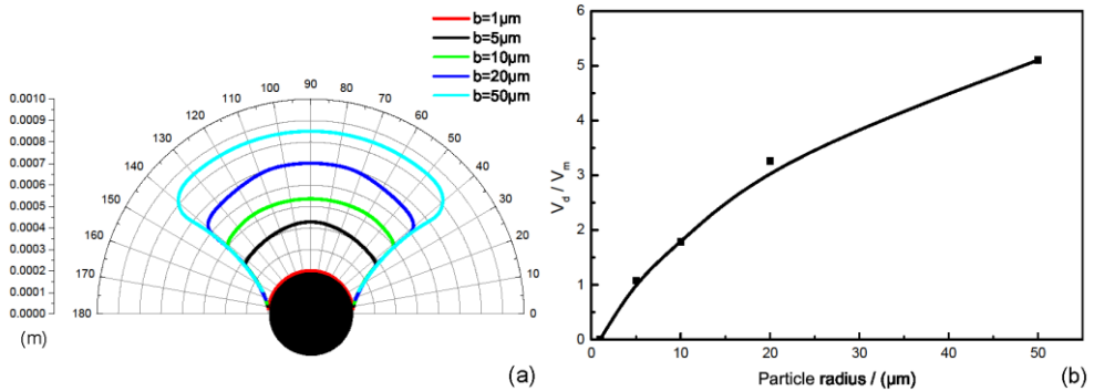
Fig. 3. Saturated buildup of particles of different sizes: magnetic induction B_0 = 0.5 \text{ T} , matrix radius a = 0.2 \text{ mm} , fluid velocity V_0 = 0.1 \text{ m/s}
