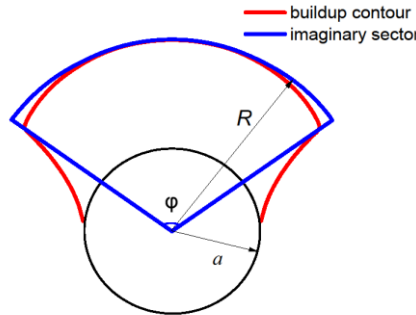
Fig. 2. Schematic diagram of imaginary sector of buildup contour
