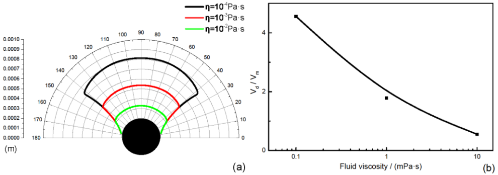
Fig. 5. Effect of the fluid viscosity on the saturated particle buildup: magnetic induction B_0 = 0.5 \text{ T} , matrix radius a = 0.2 \text{ mm} , particle radius b = 10 \mu\text{m}
