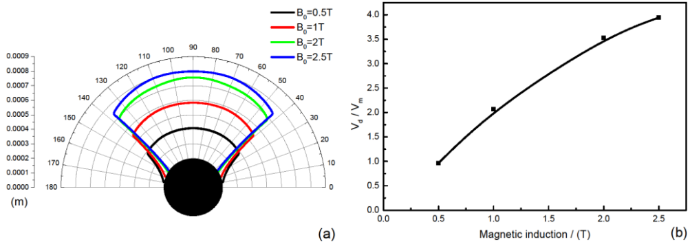
Fig. 4. Influence of the applied magnetic field strength on saturated buildup of particles: particle radius b = 5 \mu\text{m} , matrix radius a = 0.2 \text{ mm} , fluid velocity V_0 = 0.1 \text{ m/s} .
