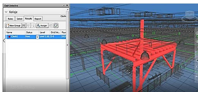
Fig. 5. Detected collision between the production place and the hall construction element.
