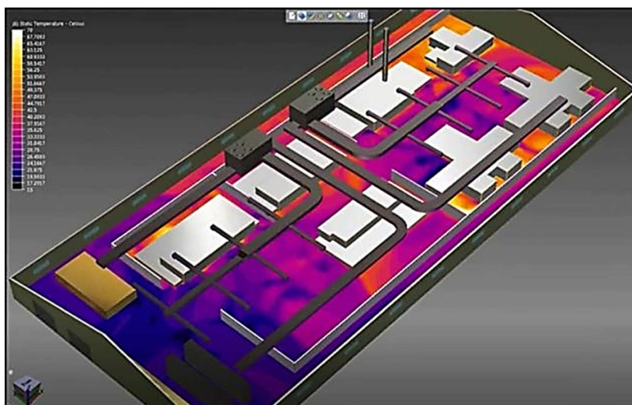
Fig. 7. Thermal analysis of the production hall.
