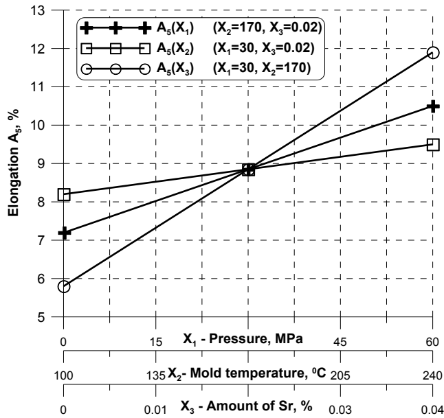
Fig. 2. The influence of squeeze pressure, mould temperature, and quantity of modifier on the elongation A_5 of castings made of AlSi7Mg alloy
