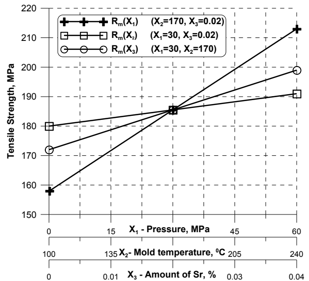
Fig. 1. The influence of squeeze pressure, mould temperature, and quantity of modifier on the tensile strength of castings made of AlSi7Mg alloy
