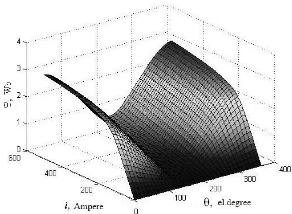
Fig. 1. Magnetizing characteristic
