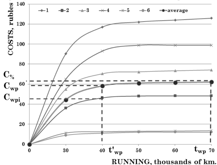
Fig. 10. A graph of the dependence of the cost of warranty repair trucks by miles. The variation of the theoretical functions of the total cost per truck for different countries: t'_{wp} – limit warranty mileage; t_{wp} – mileage warranty, the permissible value of risk
