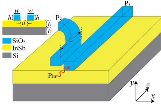
Fig. 1. Schematic diagram of THz plasmonic dielectric loaded waveguide, the inset shows the xy -plane side view of this waveguide.
