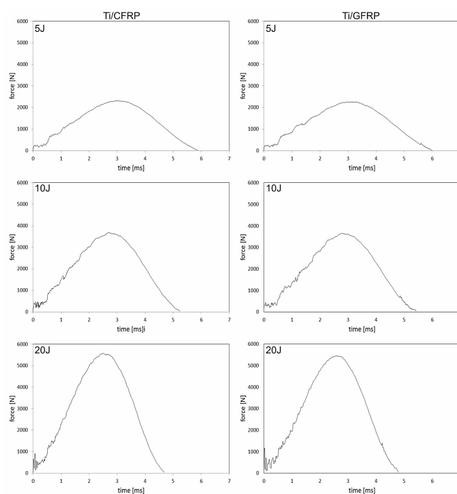
Fig. 2. Force-time curves of tested titanium-composite laminates
