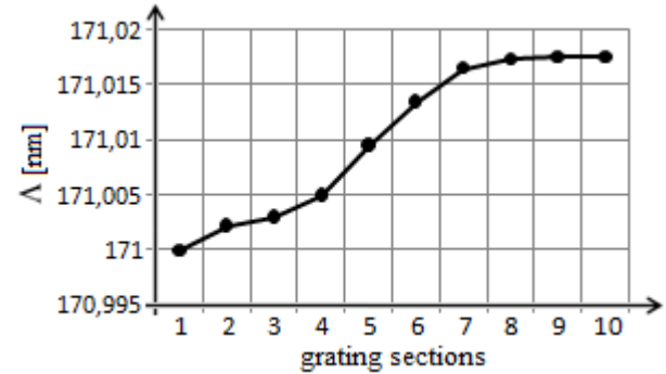
Figure 2. Change in the period length of the grating used in the dispersion compensator
