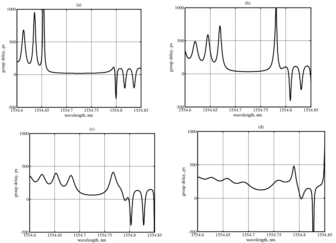
Figure 15. Graphs of group delay in the vicinity of the dispersion compensator’s Bragg wavelength, (a) no apodization, (b) Gauss apodization, a=2 , (c) Gauss apodization, a=5 , (d) Gauss apodization, a=10 ,
