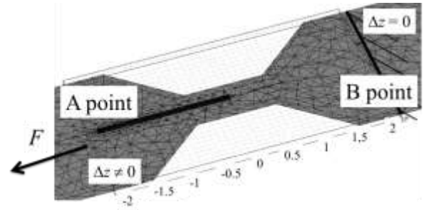
Figure 4. Grating of finished elements, applied to the dispersion compensator system consisting of a cantilever beam and Bragg grating. End A: subjected to tensile stress F , End B: firmly attached, immovable
