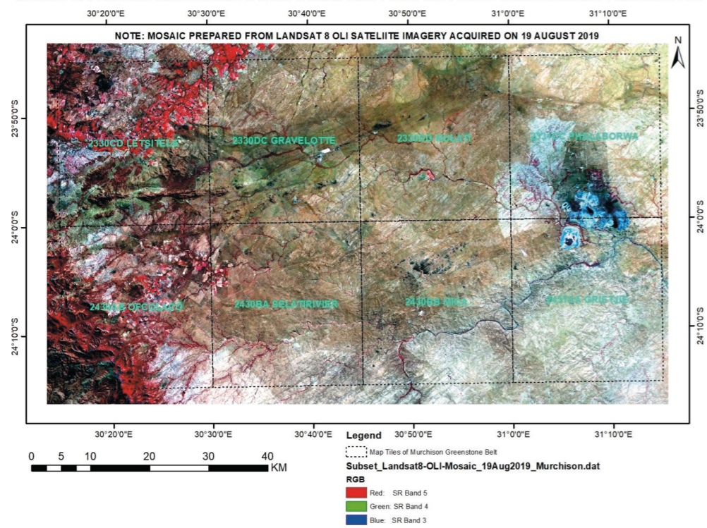
Fig. 9. Atmospherically corrected Landsat 8 level 2 product (RGB: B5-B4-B3) subsetted for eight mapping sheet areas of Murchison Greenstone Belt
