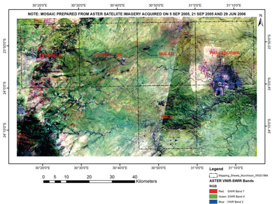
Fig. 16. Structural features and lineaments identifiable from ASTER data using FCC of RGB: B7-B4-B2 covering Murchison Greenstone Belt
