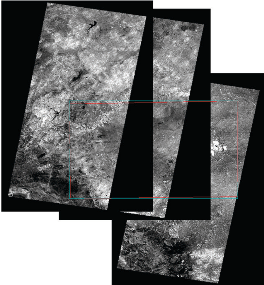
Fig. 3. Mosaics of ASTER VNIR band of adjacent scenes in the orbit direction (acquired on 5 Sep 2005, 21 Sep 2005 and 29 Jun 2006) overlaid with a polygon covering the extent of 8 mapping sheets
