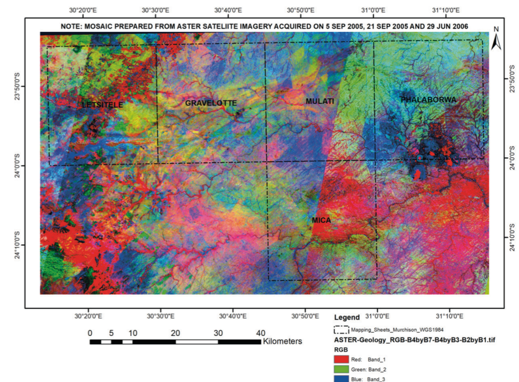
Fig. 14. Discrimination of geological features from ASTER data using FCC of RGB: B4/B7-B4/B3-B2/B1 covering Murchison Greenstone Belt
