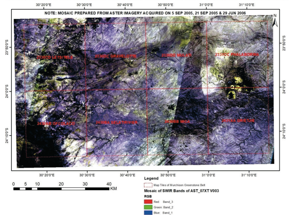
Fig. 6. FCC of Mosaicked and stacked ASTER SWIR data (acquired on 5 Sep 2005, 21 Sep 2005 and 29 Jun 2006) covering eight mapping sheets of Murchison Greenstone Belt area
