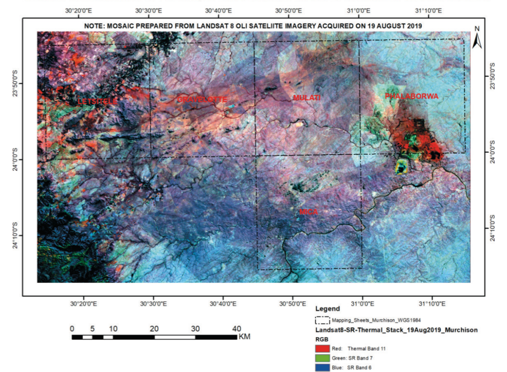
Fig. 20. Geology discrimination identifiable from Landsat 8 data using FCC of RGB: B11-B7-B6 covering Murchison Greenstone Belt
