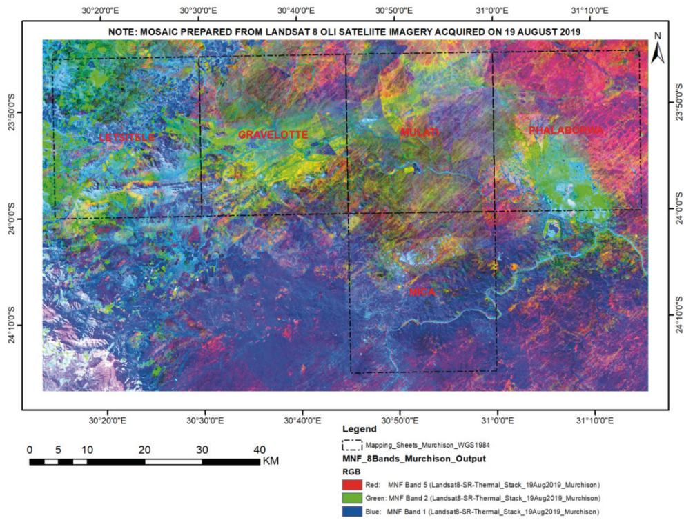
Fig. 24. Lithology and structures identifiable from MNF bands of Landsat 8 (RGB: MNF 5-MNF 2-MNF 1) covering Murchison Greenstone Belt
