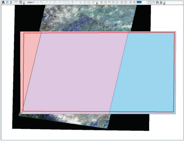
Fig. 4. Subset polygons digitised for mosaicking different ASTER scene stacks overlaid with a stack of mosaicked SWIR bands of two adjacent scenes (scenes IDs: 25492 & 25491 acquired on 21 Sep 2005)
