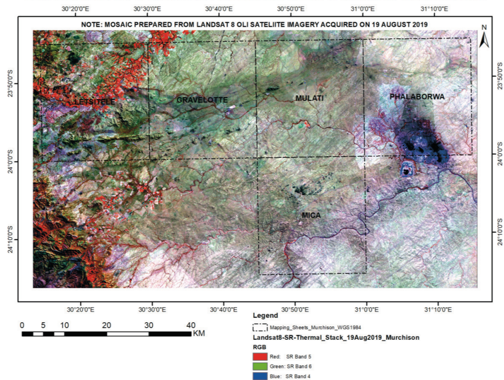
Fig. 10. Land/water display of Landsat 8 OLI dataset covering Murchison Greenstone Belt area
