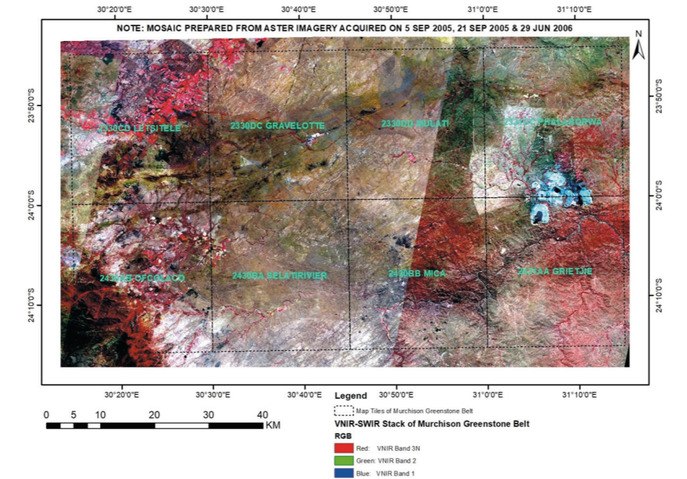
Fig. 7. FCC of Mosaicked and stacked ASTER VNIR-SWIR data (acquired on 5 Sep 2005, 21 Sep 2005 and 29 Jun 2006) covering eight mapping sheets of Murchison Greenstone Belt area
