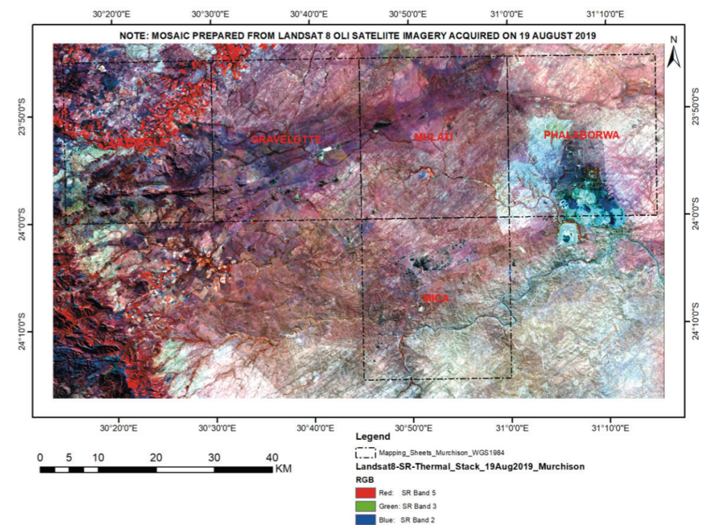
Fig. 23. Lithology and structures identifiable from Landsat 8 data using FCC of RGB: B5-B3-B2 covering Murchison Greenstone Belt
