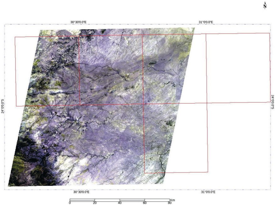
Fig. 5. Mosaicked ASTER SWIR stack of 21 Sep 2005 subsetting in ArcMap using the Clip tool (scenes IDs: 25492 & 25491 acquired on 21 Sep 2005) overlaid with five mapping sheets of Murchison Greenstone Belt area
