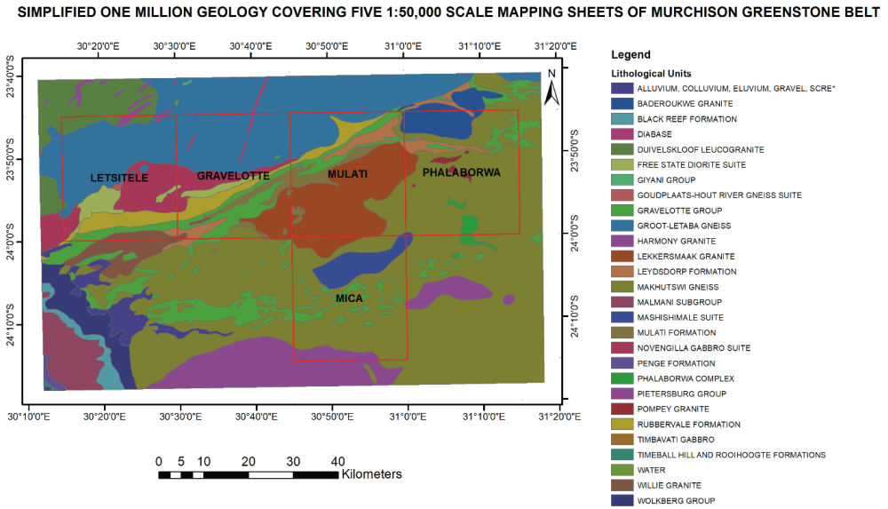
Fig. 2. Map showing the simplified geology of Murchison Greenstone Belt area (extracted from one million geological map)
