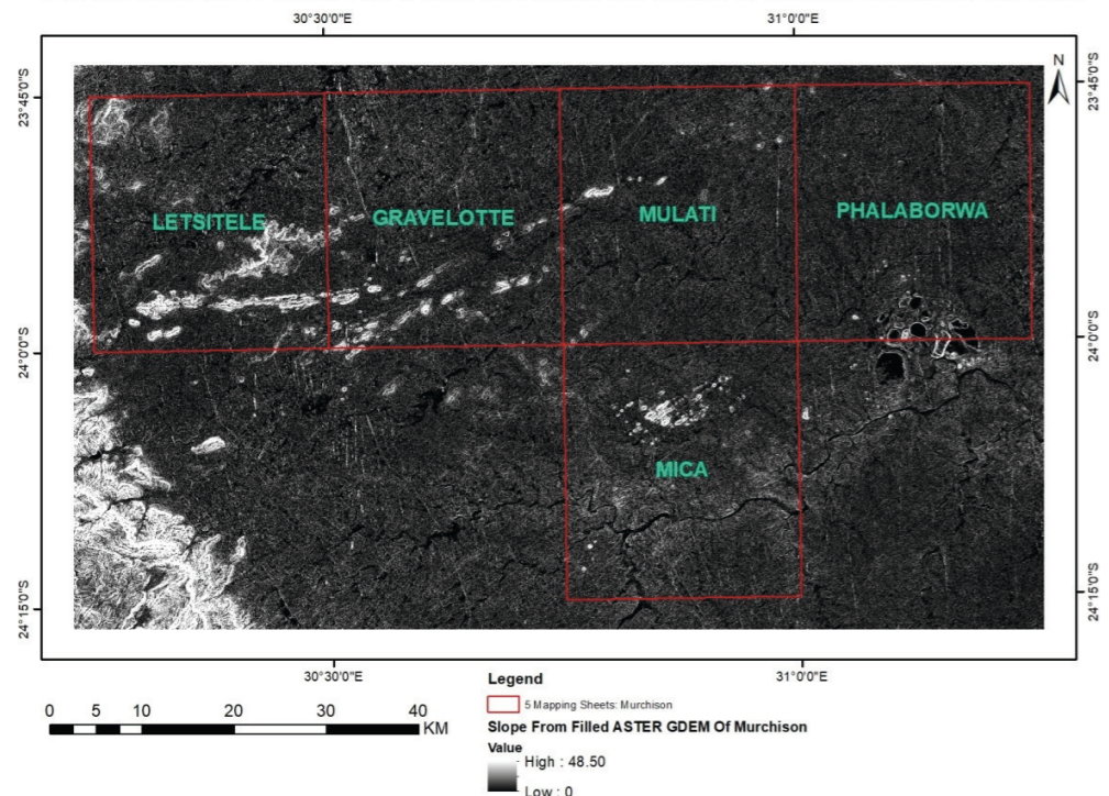
Fig. 12. Slope in degrees derived from ASTER Global Digital Elevation Model (GDEM) covering five mapping sheets of Murchison Greenstone Belt
