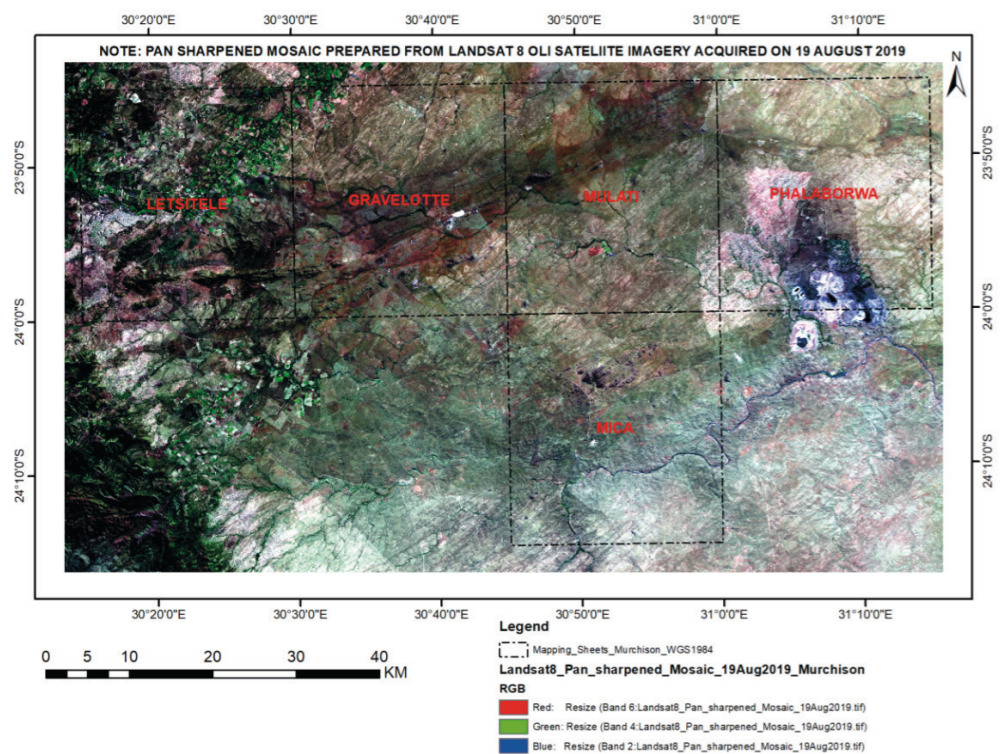
Fig. 21. Lithology and structures identifiable from PAN-sharpened bands of Landsat 8 (RGB: PS_B6-PS_B4-PS_B2) covering Murchison Greenstone Belt
