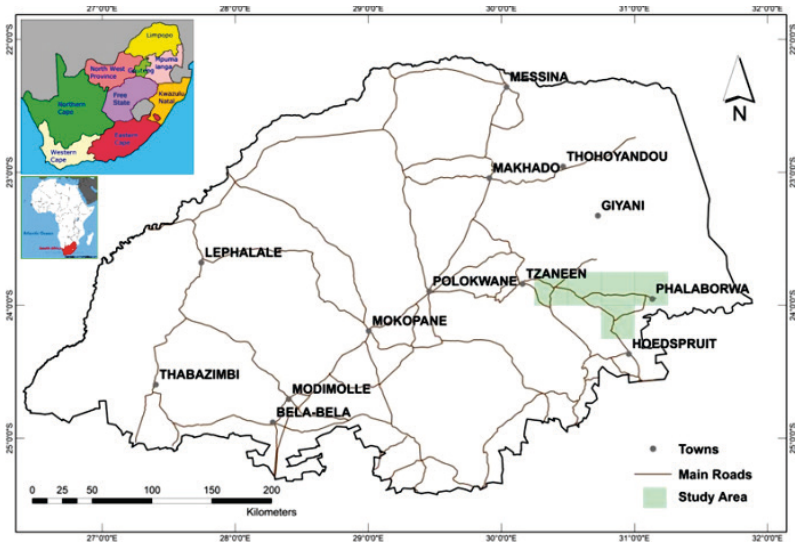
Fig. 1. Map showing the location and extent of five mapping sheets (1:50,000 scale) of Murchison Greenstone Belt area within the Limpopo Province of South Africa
