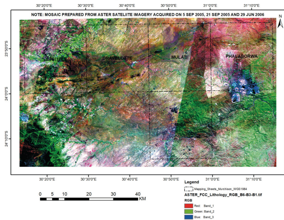
Fig. 15. Discrimination of lithology and geological features from ASTER data using FCC of RGB: B6-B3-B1 covering Murchison Greenstone Belt
