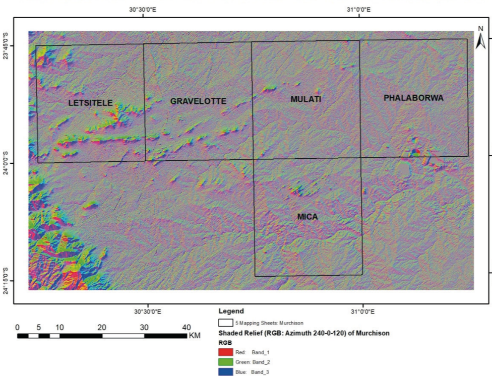
Fig. 13. Shaded relief in RGB: 240-0-120 degrees derived from ASTER DEM for five mapping sheets Murchison Greenstone Belt
