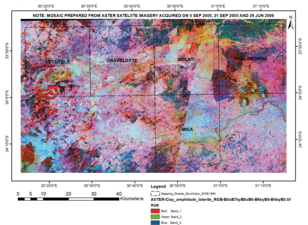
Fig. 18. Clay, amphibole and laterite identifiable from ASTER data (FCC of RGB: B5xB7)/B6xB6-B6/B8-B4/B5 covering Murchison Greenstone Belt)
