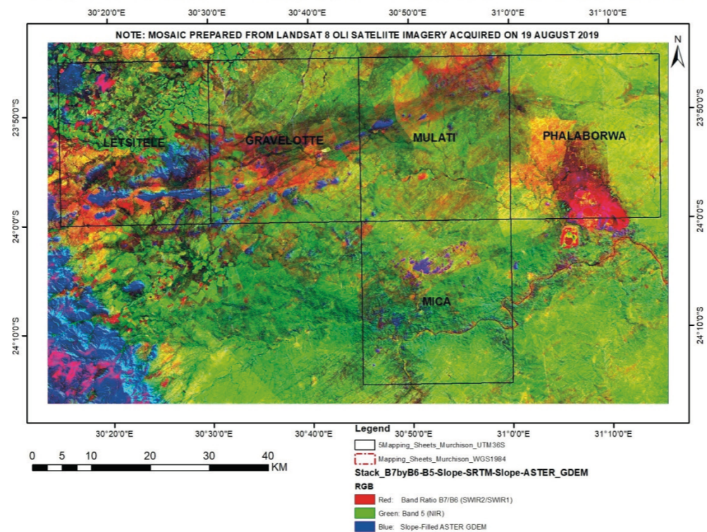
Fig. 22. Lithology and structures identifiable from Landsat 8 bands and slope (RGB: B7/B6-B5-Slope) covering Murchison Greenstone Belt
