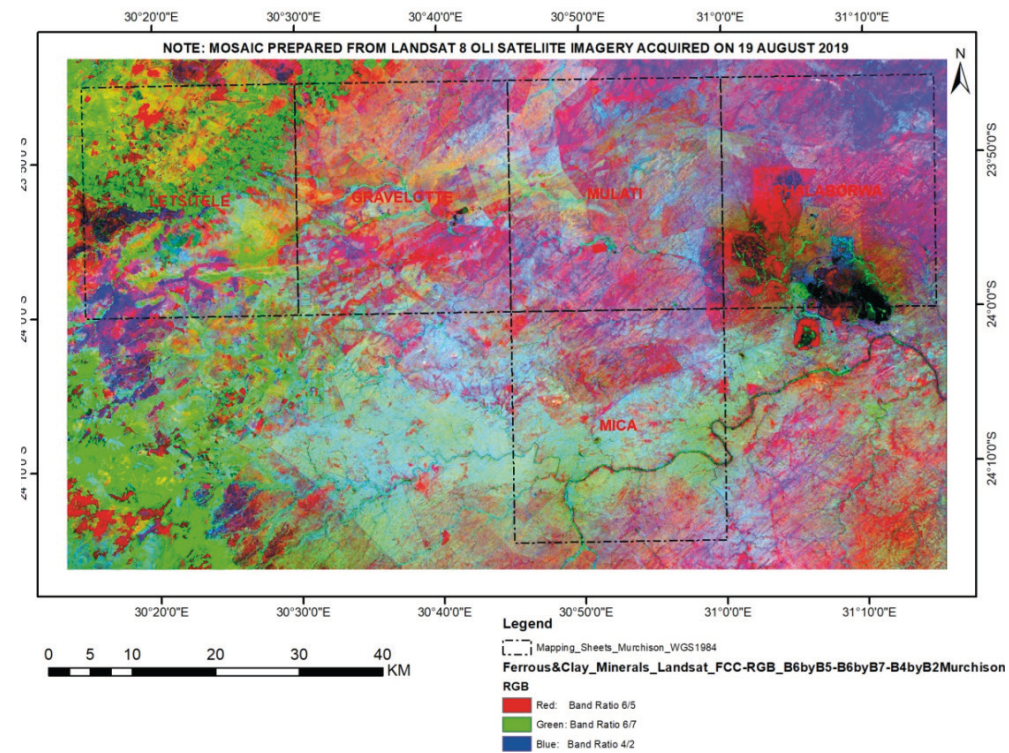
Fig. 26. Ferrous and clay minerals identifiable from Landsat 8 data using FCC of RGB: B6/B5-B6/B7-B4/B2 covering Murchison Greenstone Belt
