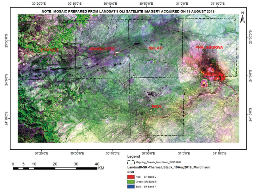
Fig. 25. Iron oxides and clay minerals identifiable from Landsat 8 data using FCC of RGB: B2-B5-B7 covering Murchison Greenstone Belt
