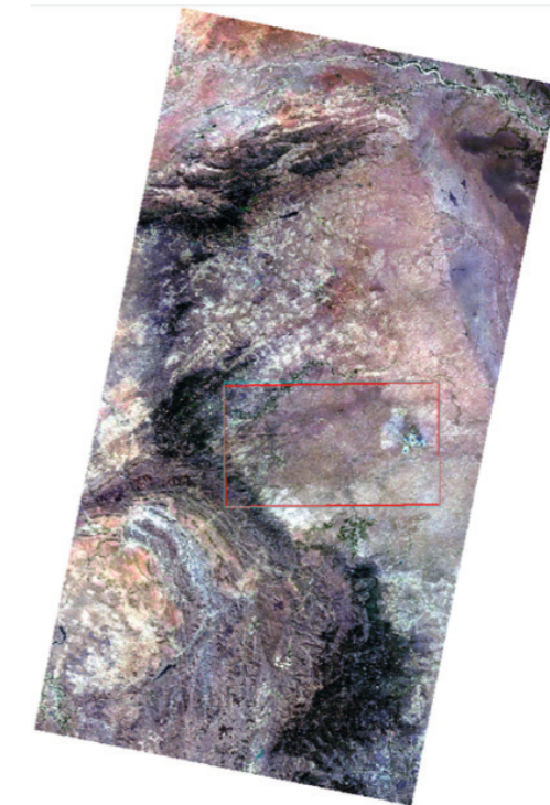
Fig. 8. Mosaic of atmospherically corrected true colour Landsat 8 OLI level 2 product overlaid with a polygon covering 8 mapping sheets
