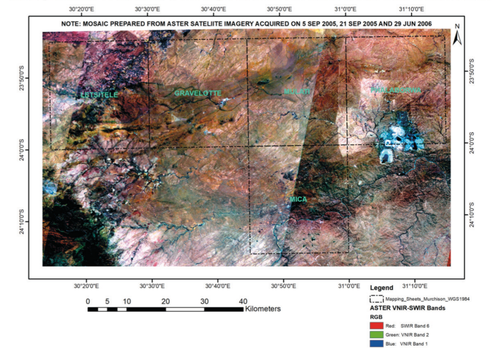
Fig. 17. Goossan, alteration and host rocks identifiable from ASTER data using FCC of RGB: B6-B2-B1 covering Murchison Greenstone Belt
