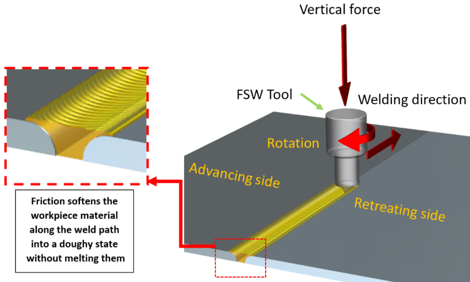
Fig. 1. Scheme of FSW process
