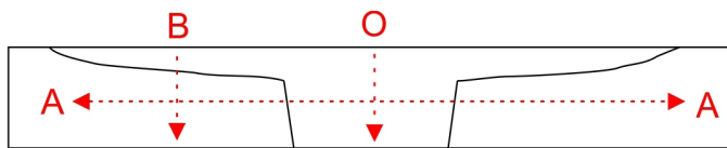
Fig. 11. Scheme of hardness measurement areas
