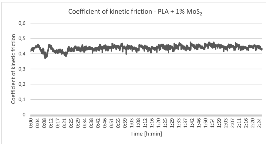
Fig. 5. Values of the kinetic friction coefficient during the whole test – PLA + 1% MoS 2
