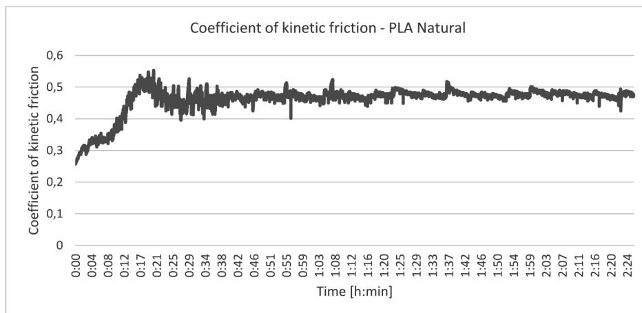
Fig. 7. Values of the kinetic friction coefficient during the whole test – PLA Natural printed
