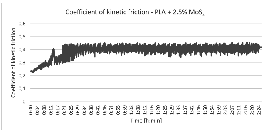
Fig. 6. Values of the kinetic friction coefficient during the whole test – PLA + 2.5% MoS 2
