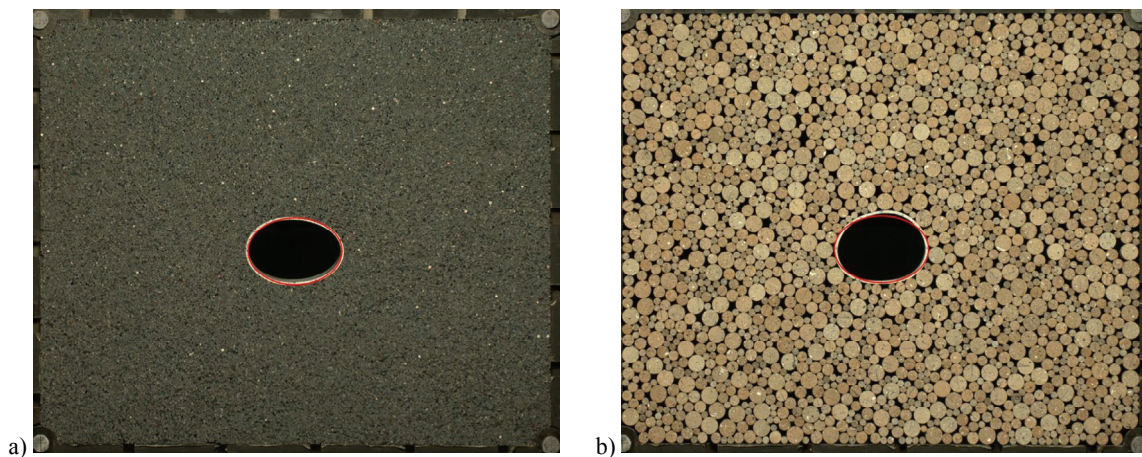
Fig. 5. Images of the loaded samples. A red ellipse with the same value of eccentricity was superposed over each pipe (a) PVC rods; (b) Wooden rods
