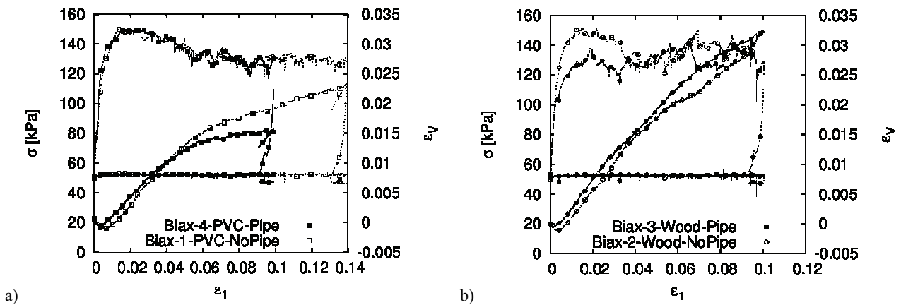
Fig. 4. 1\gamma 2\varepsilon experiment results of two types of materials with or without a circular, flexible pipe inside.
