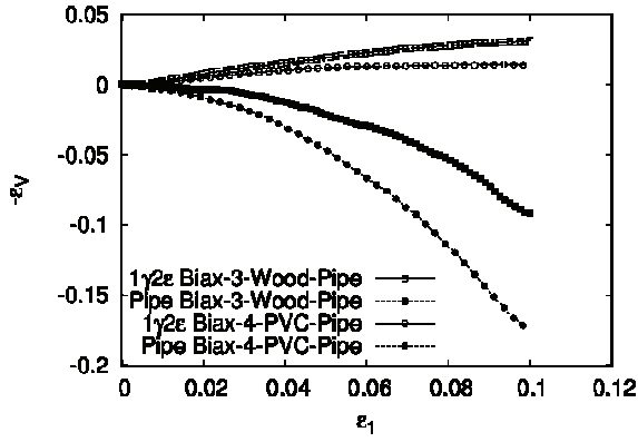
Fig. 6. During vertical compression test in 1\gamma 2\epsilon the volumetric strains of the apparatus and the pipe specimen were different. The whole sample was dilating ( \epsilon_V > 0 , top two curves) while the PVC pipe was contracting ( \epsilon_V < 0 , bottom two curves)
