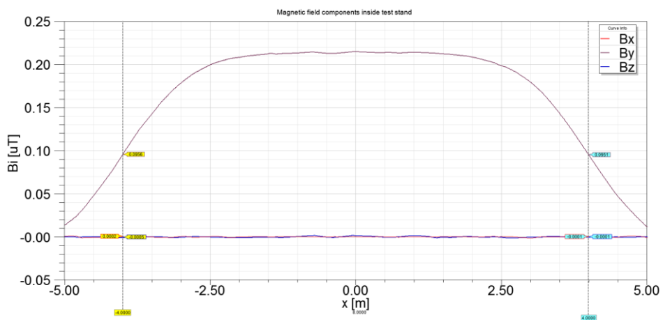
Fig. 21. B_y component generated by test stand
