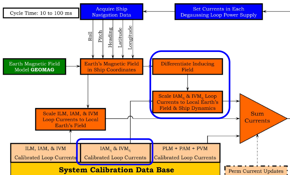
Fig. 30. DG with eddy current magnetic signature reduction module [13]
