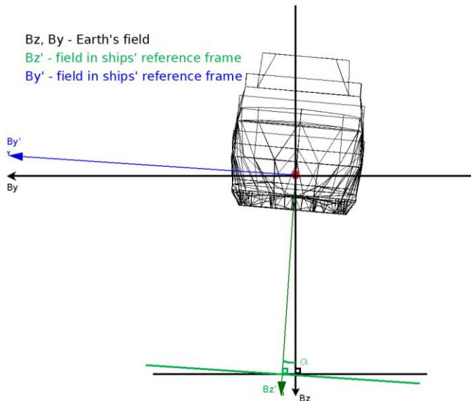
Fig. 6. Ship shown from stern on E-W course
