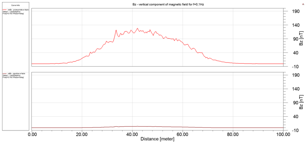
Fig. 17. Vertical component: quadrature (top) and in phase (bottom) for f = 0.1 Hz
