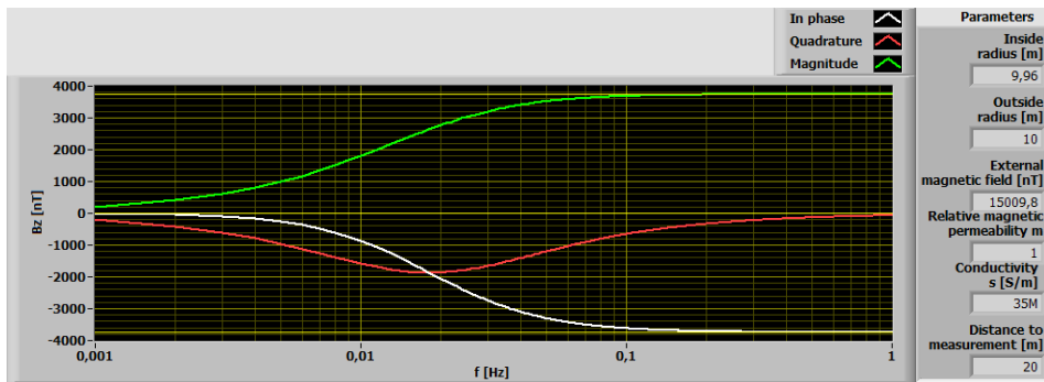
Fig. 8. Model results for \mu_r = 1, \sigma = 35 \text{ MS/m} , aluminium
