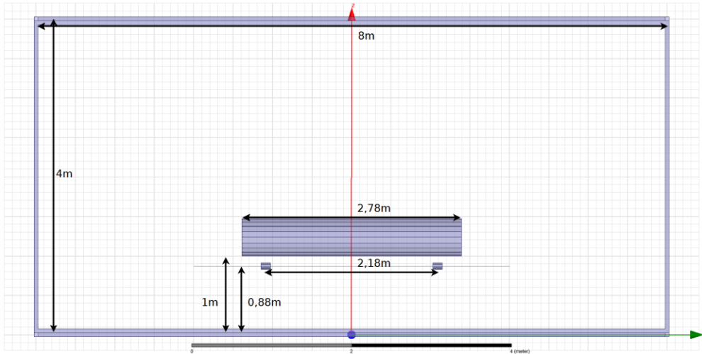
Fig. 25. Schematic drawing of simplified model in test stand
