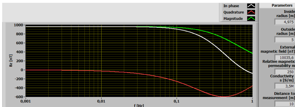
Fig. 13. Off board loop effect for coils inside conducting hull — analytical model
