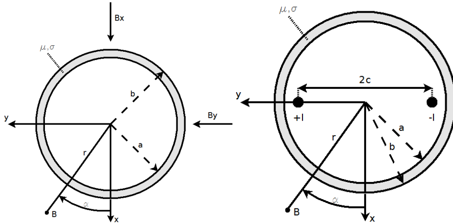
Fig. 5. Analytical model geometry: ship's hull (left); hull with loop (right)
