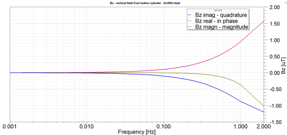
Fig. 12. FEA results for \mu_r = 1.003 , \sigma = 1.1 MS/m, AL6XN steel
