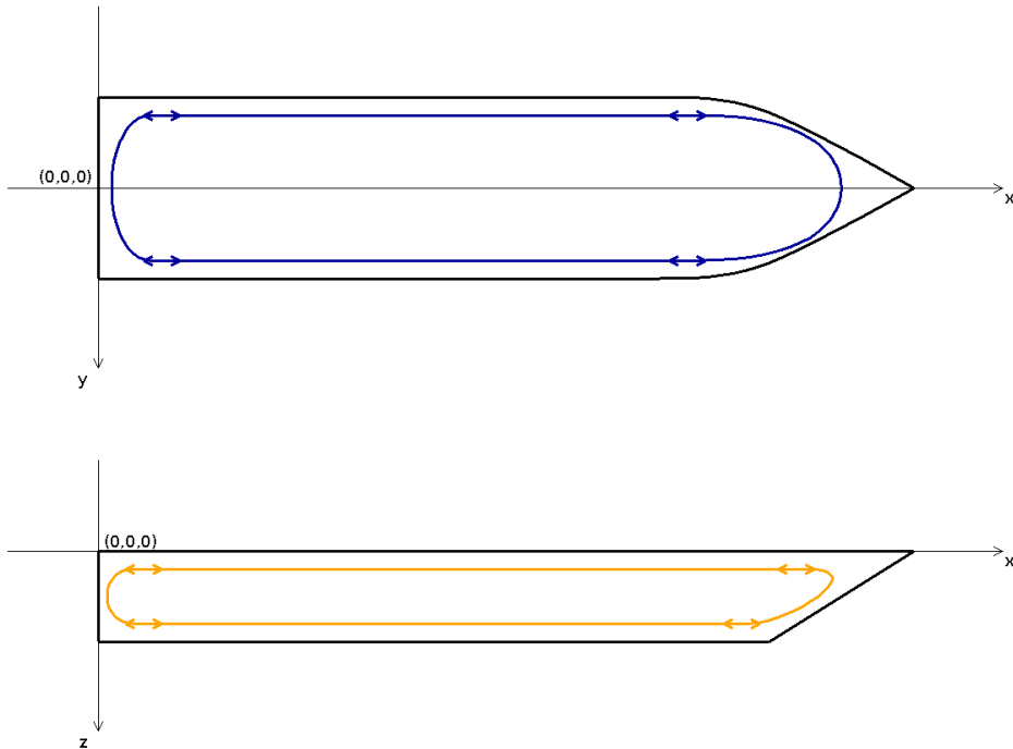
Fig. 1. Eddy currents in ship's hull due to its roll
