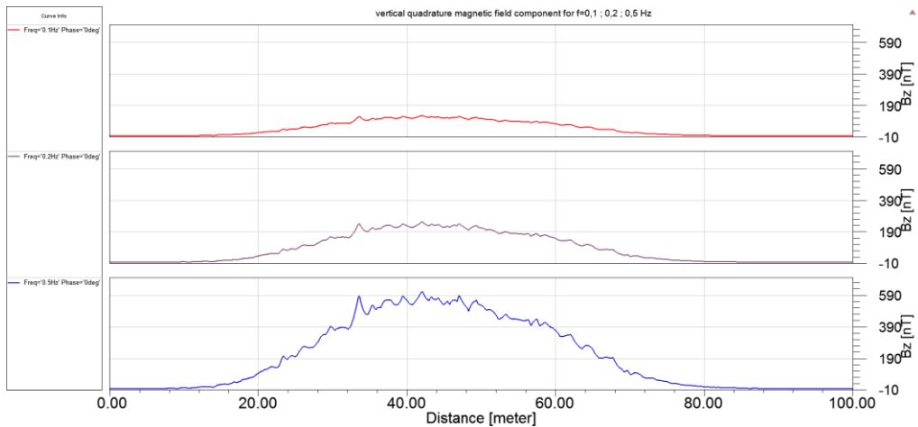
Fig. 18. Quadrature vertical component for f = 0.1 Hz (top), 0.2 Hz (middle) and 0.5 Hz (bottom)
