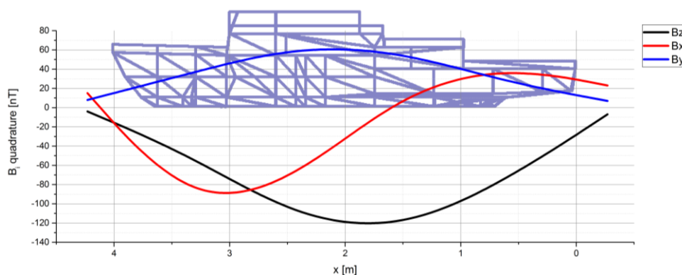
Fig. 29. Example secondary fields @ 40 Hz (middle) and hull screening effect for one of the coils (bottom) — which for the PSM is negligible (in accordance with calculations)
