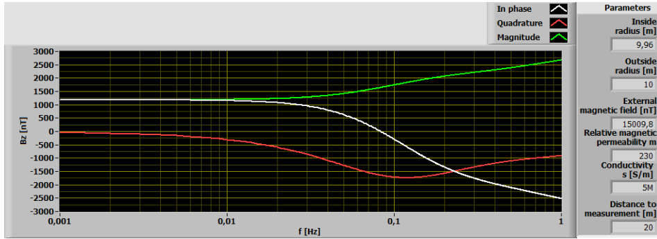
Fig. 7. Model results for \mu_r = 230, \sigma = 5 \text{ MS/m} , HSS steel
