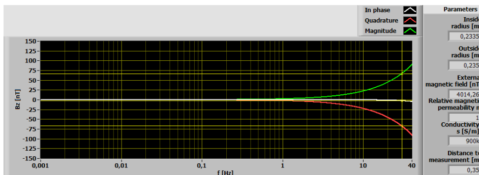
Fig. 28. Analytical model results for simplified model case
