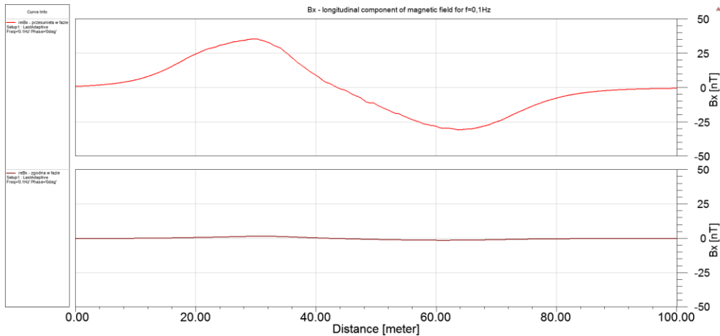
Fig. 16. Longitudinal component: quadrature (top) and in phase (bottom) for f = 0.1 Hz
