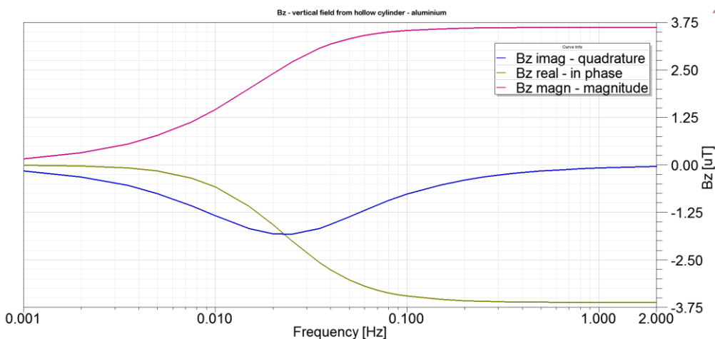
Fig. 11. FEA results for \mu_r = 1 , \sigma = 35 MS/m, aluminium
