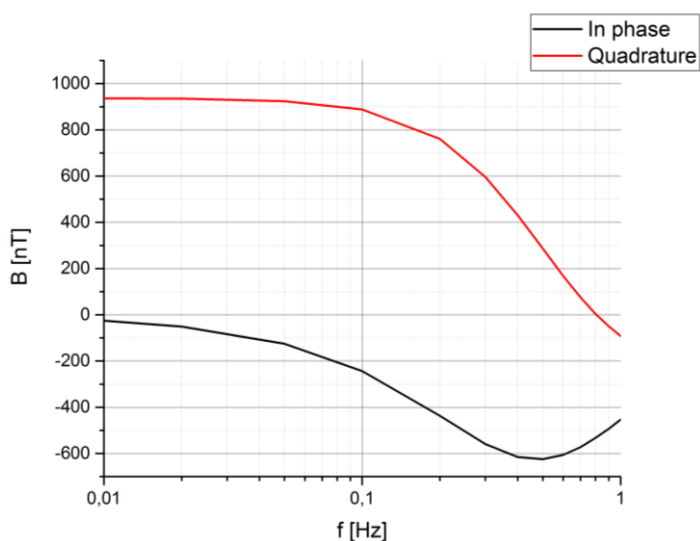
Fig. 14. Off board loop effect for coils inside conducting hull — FE model (in phase — red, quadrature — black)
