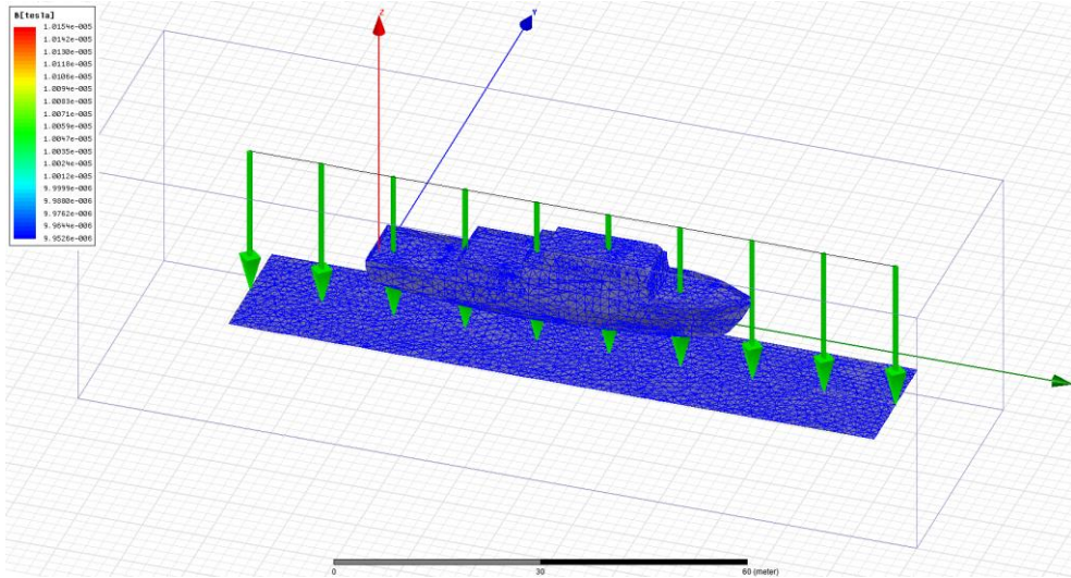
Fig. 15. Ship's model in vertical external field
