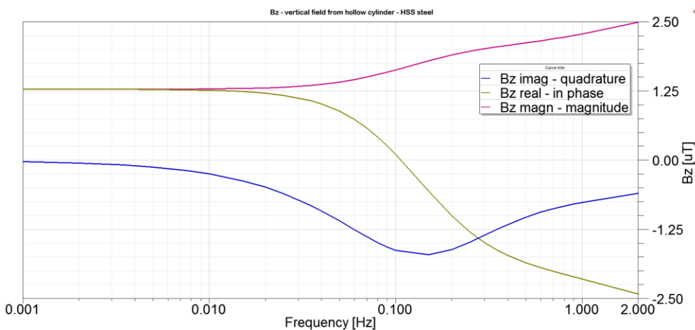
Fig. 10. FEA results for \mu_r = 230 , \sigma = 3.5 MS/m, HSS steel
