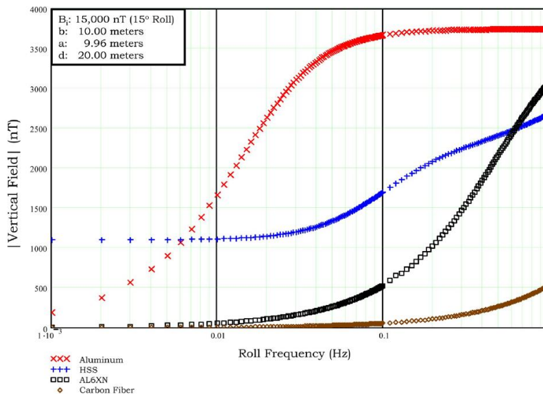
Fig. 2. Eddy current magnetic field magnitude from conducting cylinder made of different materials [13]
