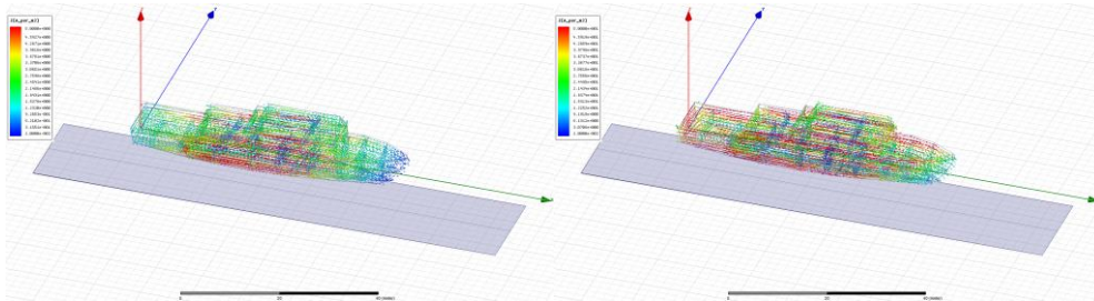
Fig. 19. In phase current density ( j_{maks} = 5 \text{ A/m}^2 ) (left), quadrature current density for f = 0.2 \text{ Hz} ( j_{maks} = 50 \text{ A/m}^2 ) (right)
