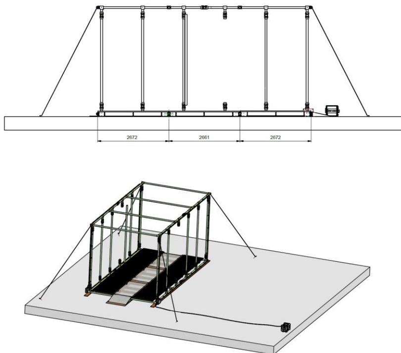
Fig. 20. Schematic drawing of test stand
