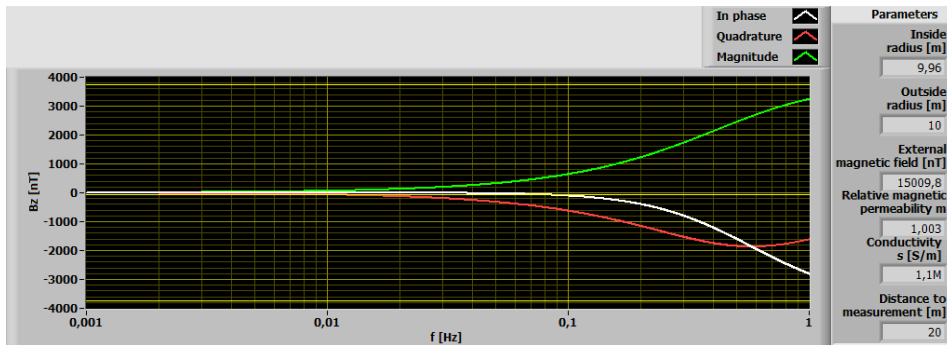
Fig. 9. Model results for \mu_r = 1.003, \sigma = 1.1 \text{ MS/m} , AL6XN steel
