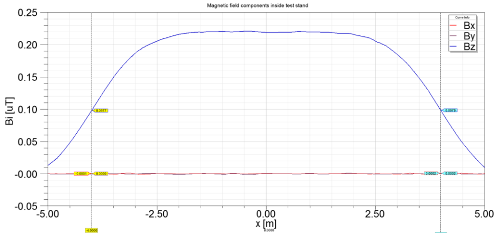
Fig. 22. B_z component generated by test stand
