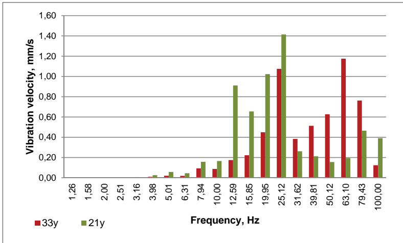
Fig. 6. Comparison of vibration structures – test stands 33 and 21
