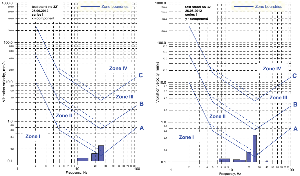
Fig. 12. Assessment of vibration impact on protected structures – series I – test stand No. 32'
