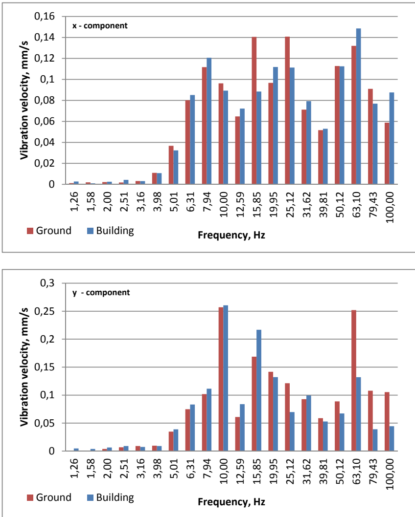
Fig. 16. The octave analysis of vibrations registered at test stands No. 34 and 34' – series III
