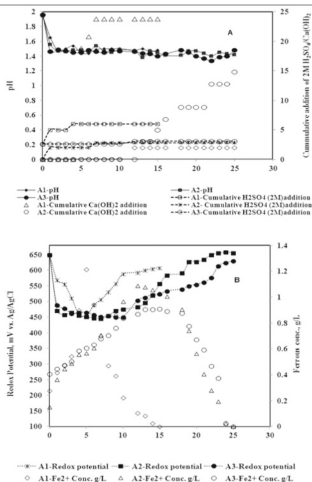
Figure 2. The plot of (A) pH and cumulative addition of 2M H 2 SO 4 /Ca(OH) 2 versus time (B) redox potential (mV) and ferrous concentration (g L -1 ) versus time
