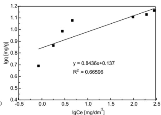
Fig. 8. Freundlich isotherm of uranium biosorption on rice husk (adsorbent dose – 8 g/dm 3 , pH = 3, t = 60 min, T = 298 K, rice husk size – 150 \mu\text{m} )
