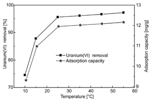
Fig. 6. Effect of temperature on uranium biosorption by rice husk (adsorbent dose – 8 \text{g}/\text{dm}^3 , \text{pH}=3 , t=60 min, rice husk size –150 \mu\text{m} , initial uranium concentration – 100 \text{mg}/\text{dm}^3 )
