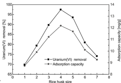
Fig. 5. Effect of rice husk size (in \mu\text{m} ) on uranium biosorption: 1) 250–380, 2) 80–250, 3) 150–180, 4) 120–150, 5) 109–120, 6) 96–109, 7) 80–96 (adsorbent dose – 8 \text{g/dm}^3 , pH = 3, t = 60 min, T = 25 °C, initial uranium(VI) concentration – 100 \text{mg/dm}^3 )
