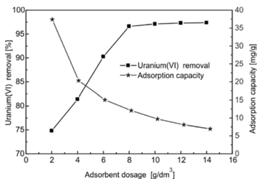
Fig. 4. Effect of adsorbent dosage on uranium biosorption by rice husk (pH = 3, t = 60 min, T = 25 °C, rice husk size – 150 \mu\text{m} , initial uranium(VI) concentration – 100 \text{mg/dm}^3 )
