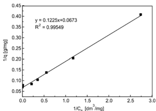
Fig. 7. Langmuir isotherm of uranium biosorption on rice husk (adsorbent dose – 8 g/dm 3 , pH = 3, t = 60 min, T = 298 K, rice husk size – 150 \mu\text{m} )
