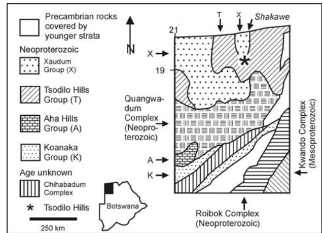
Fig. 2. Precambrian units in NW Botswana (modified from Carney et al. , 1994; Key & Mothibi, 1999; Key & Ayers, 2000; Singletary et al. , 2003)
