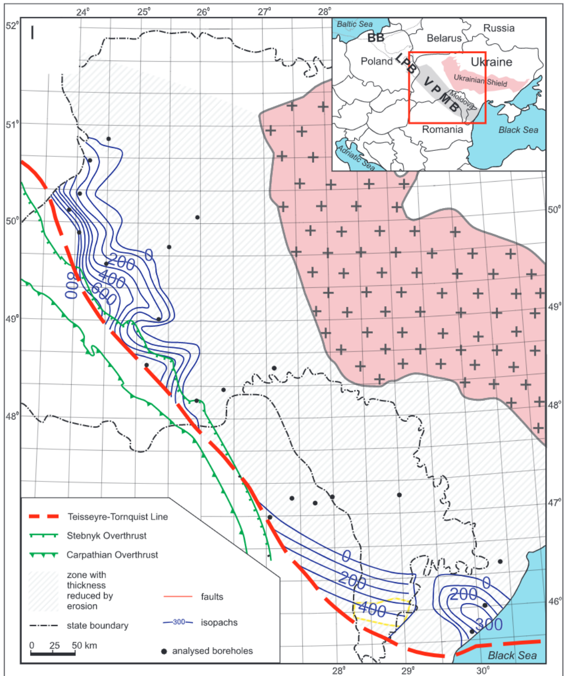
Fig. 6I – thickness maps for the following stratigraphic and lithostratigraphic units of the Volyn-Podillya-Moldavia Basin
