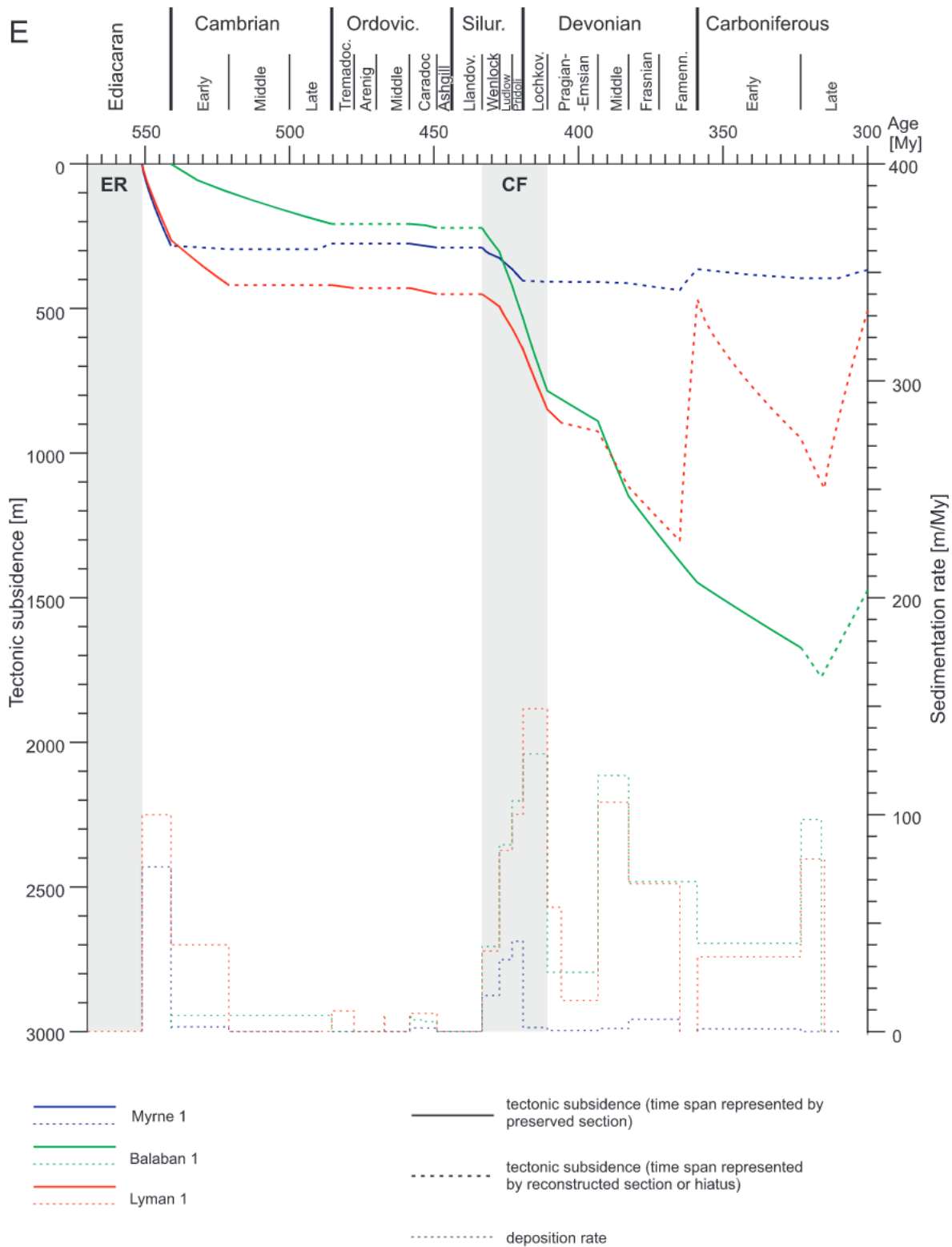
Fig. 5E – results of backstripping: tectonic subsidence curves and sedimentation rate diagrams for 21 boreholes from the Volyn-Podillya-Moldavia Basin (ER – Ediacaran rifting, locally with rift-related magmatic activity, CF – Caledonian foredeep)
