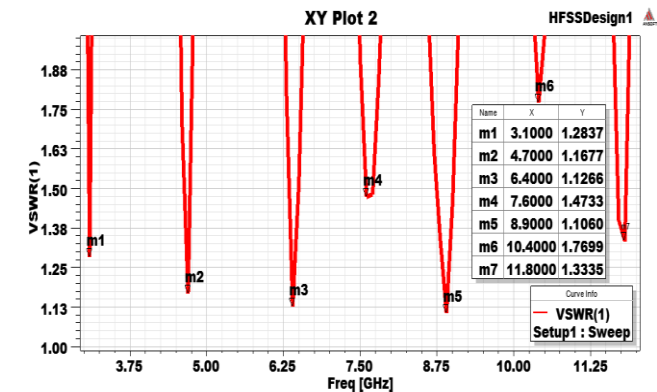
Fig. 6. VSWR plot of the proposed antenna
