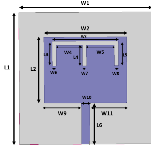
Fig. 1. Physical layout of the proposed antenna
