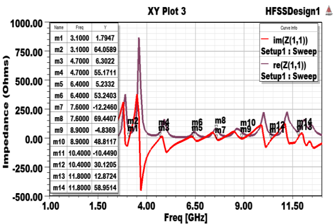
Fig. 7. Simulated input impedance
