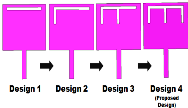
Fig. 2. Evolution steps of the proposed antenna structure.
