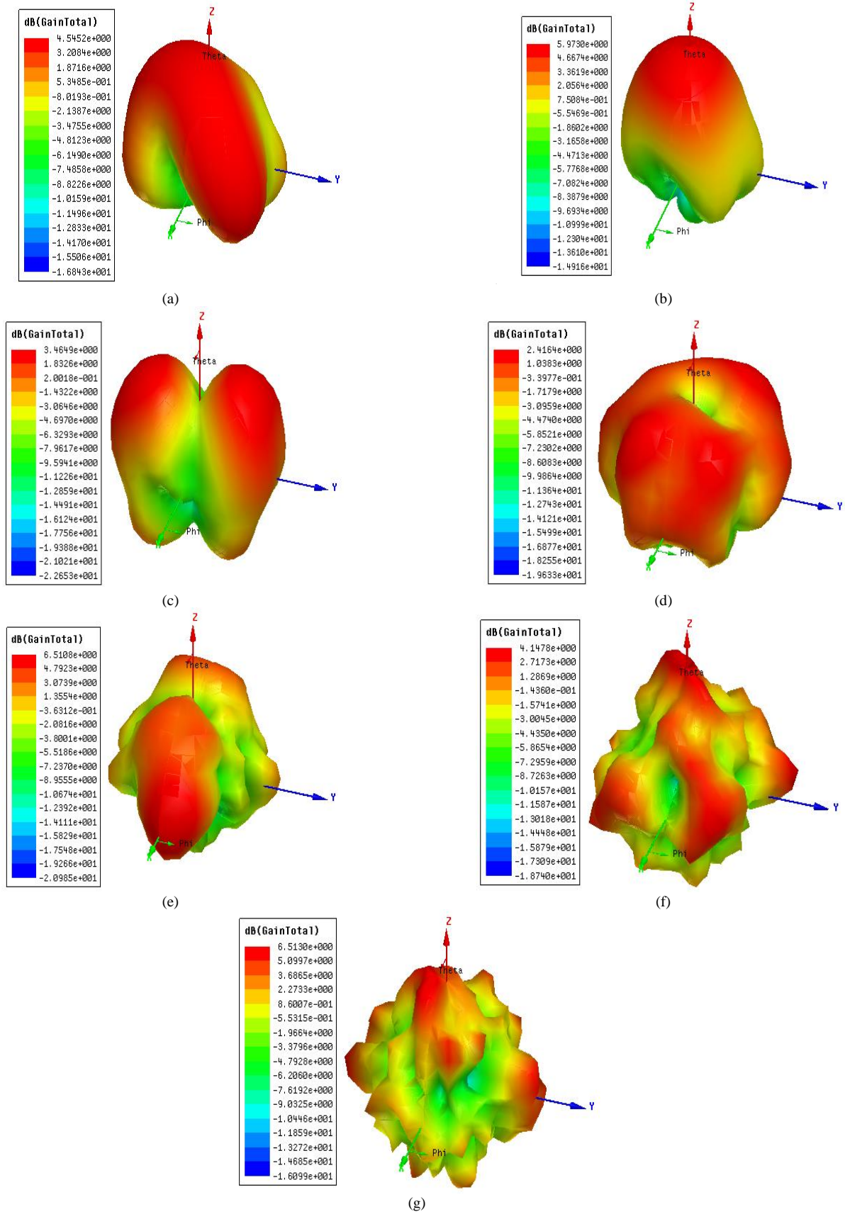
Fig. 9. Simulated at (a) 3.1, (b) 4.7, (c) 6.4, (d) 7.6, (e) 8.9,(f) 10.4 and (g) 11.8 GHz
