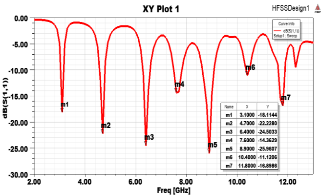
Fig. 5. Simulated S_{11} (reflection coefficient) of the proposed design
