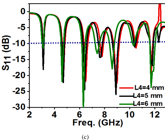
Fig. 4. Parametric study of (a) L_3 , (b) L_5 and (c) L_4
