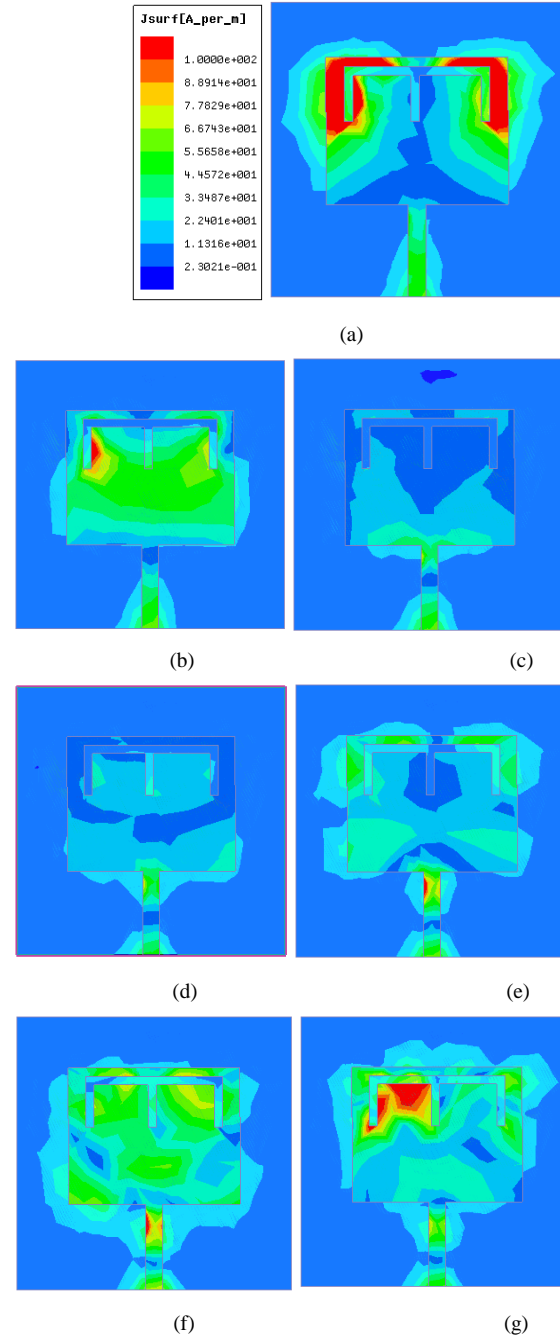
Fig. 8. Distribution of surface Current at (a) 3.1, (b) 4.7, (c) 6.4, (d) 7.6, (e) 8.9, (f) 10.4 and (g) 11.8 GHz
