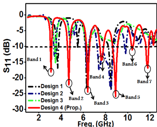
Fig. 3. Evolution design variation of S_{11} results
