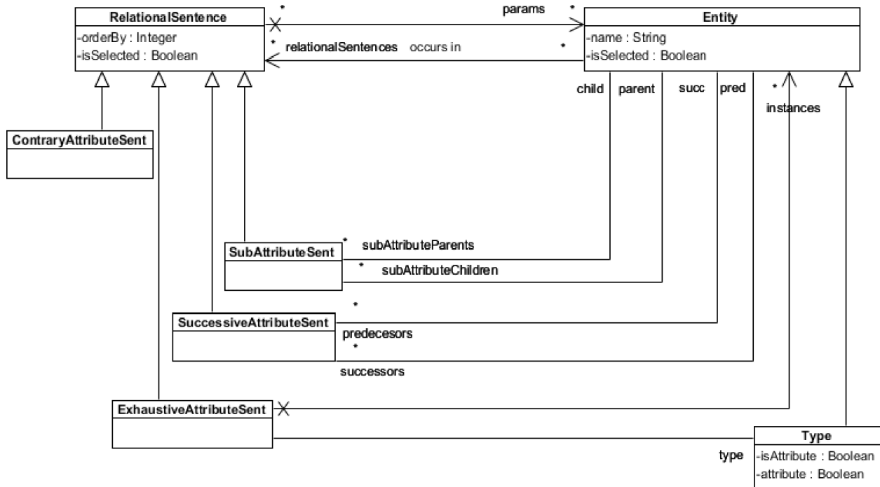
Figure 5. Extended version of SUMO meta-model – definition of attributes’ relations
