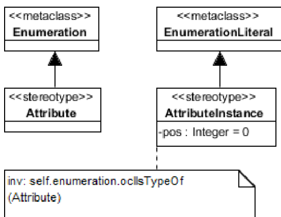
Figure 6. UML profile to represent SUMO attributes
