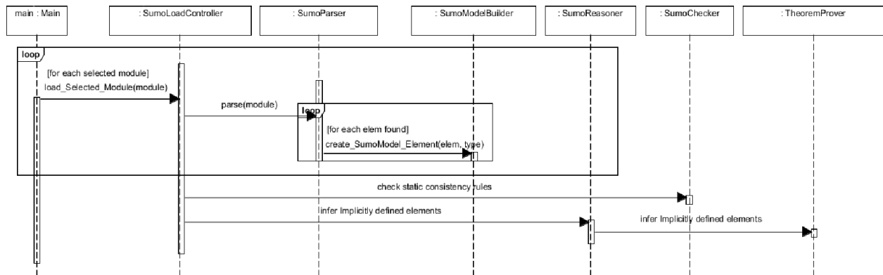
Figure 4. Processing of ontology segment
