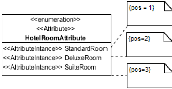
Figure 7. Transformation of successorAttribute relation
