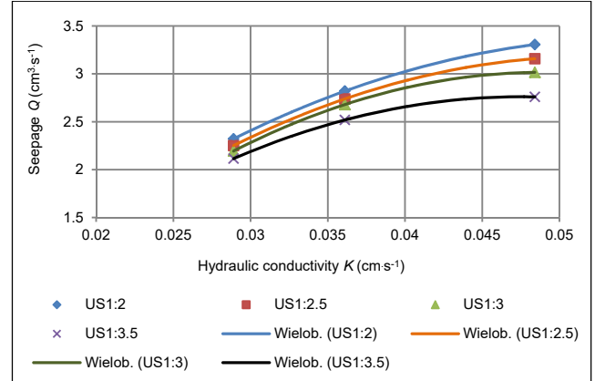
Fig. 12. Seepage and hydraulic conductivity relationship for different US slopes; source: own study
