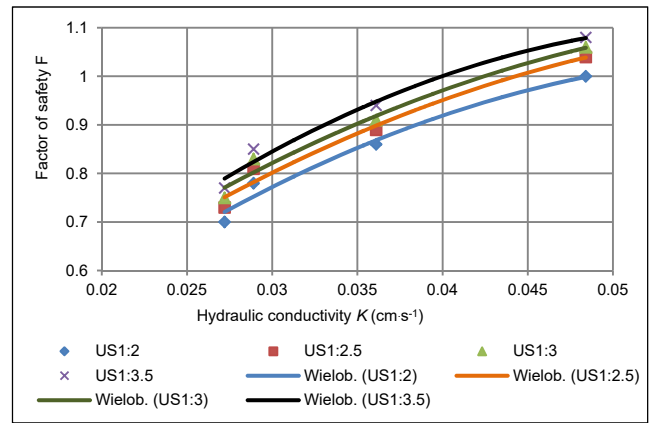
Fig. 10. The factor of safety and hydraulic conductivity relationship for different US slopes; source: own study
