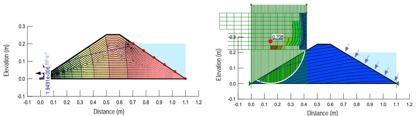
Fig. 4. Numerical analyses by GeoStudio software for soil 4 and upstream slope 1:2: a) seepage, b) factor of safety; source: own study
