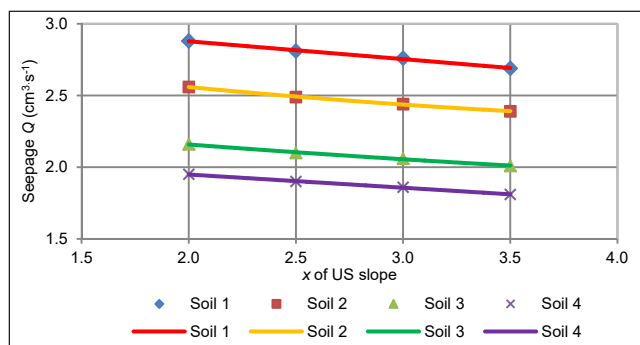
Fig. 7. Seepage and upstream (US) slope relationship for different types of soils; source: own study
