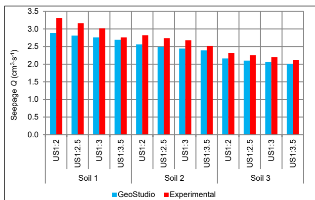
Fig. 13. Comparison of seepage for the numerical and experimental models; US = upstream slope; source: own study
