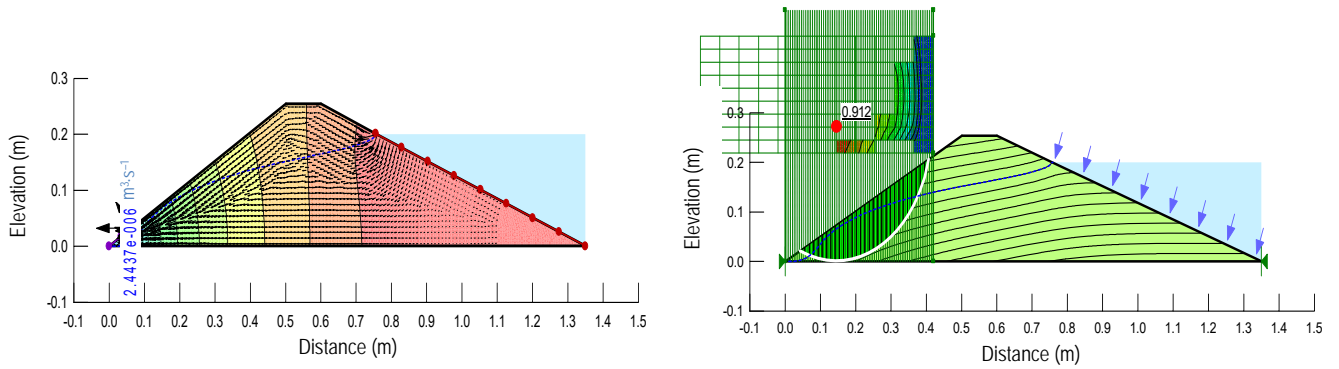
Fig. 2. Numerical analyses by GeoStudio software for soil 2 and upstream slope 1:3: a) seepage, b) factor of safety; source: own study
