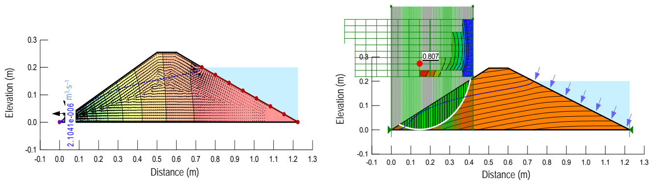
Fig. 3. Numerical analyses by GeoStudio software for soil 3 and upstream slope 1:2.5: a) seepage, b) factor of safety; source: own study
