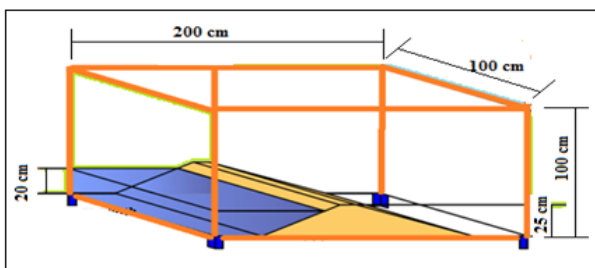
Fig. 5. Schematic diagram of the experimental model for earthfill dam; source: own study
