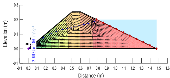
Fig. 1. Numerical analyses by GeoStudio software for soil 1 and upstream slope 1:3.5: a) seepage, b) factor of safety; source: own study
