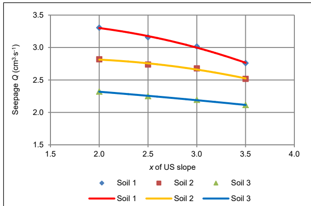
Fig. 11. Seepage and US slope relationship for different types of soils; source: own study
