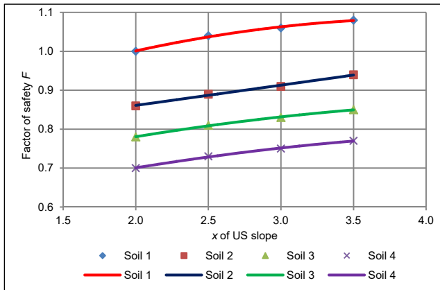
Fig. 9. The factor of safety and upperstream (US) slope relationship for different types of soils; source: own study
