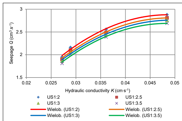
Fig. 8. Seepage and hydraulic conductivity relationship for different US slopes; source: own study
