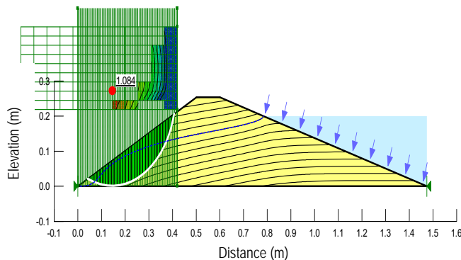
Fig. 1. Numerical analyses by GeoStudio software for soil 1 and upstream slope 1:3.5: a) seepage, b) factor of safety; source: own study
