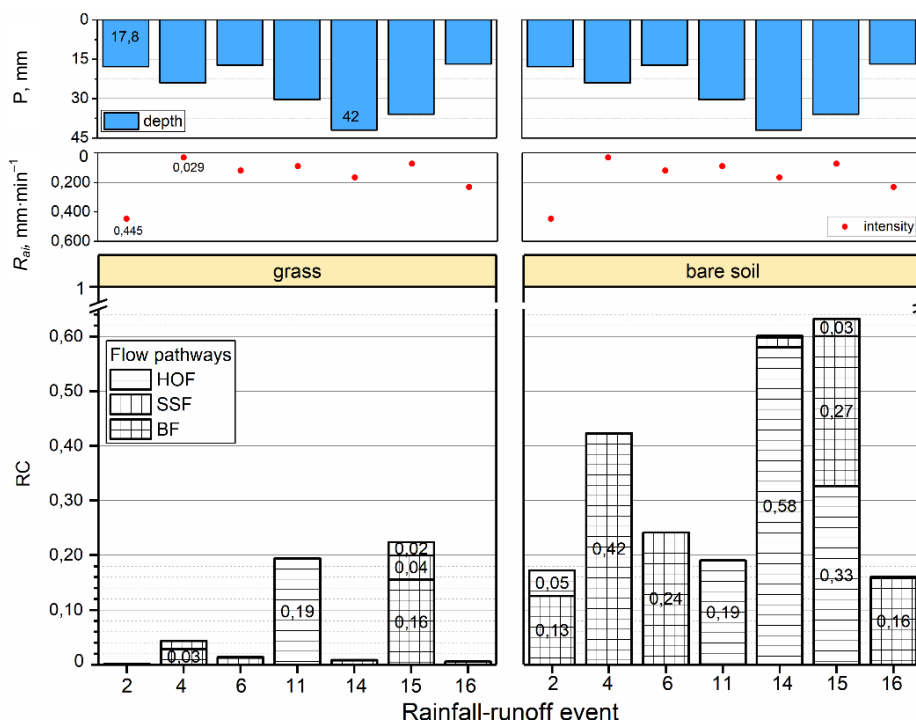
Fig. 4. Rainfall depth ( P ) and average intensity of rainfall event ( R_{ait} ), and associated runoff coefficients ( RC ), HOF = Hortonian overland flow, SSF subsurface flow, BF = base flow; note: rainfall-runoff number of events corresponds to the number from Table 4; source: own study
