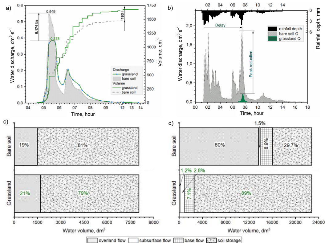
Fig. 3. Rainfall events hydrographs of discharge and volume (lag time, peak discharge, mass curve) for: a) Hortonian overland flow ( HOF ), 2.06.2016, b) HOF , 20.09.2016, c) water volume pathways on soil water balance plots ( SWBP ), 2.06.2016, d) SWBP , 20.09.2016; source: own study
