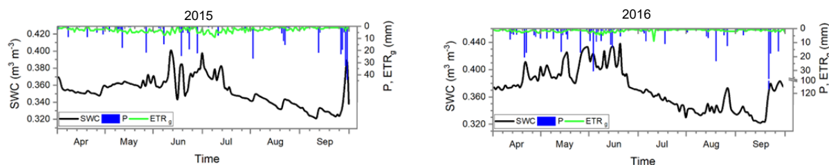
Fig. 2. Daily values of soil water content ( SWC ), rainfall ( P ) and grass evapotranspiration ( ETR_g ) during the growing season (from April 1 up to September 30) of 2015 and 2016 in VEB; source: own study
