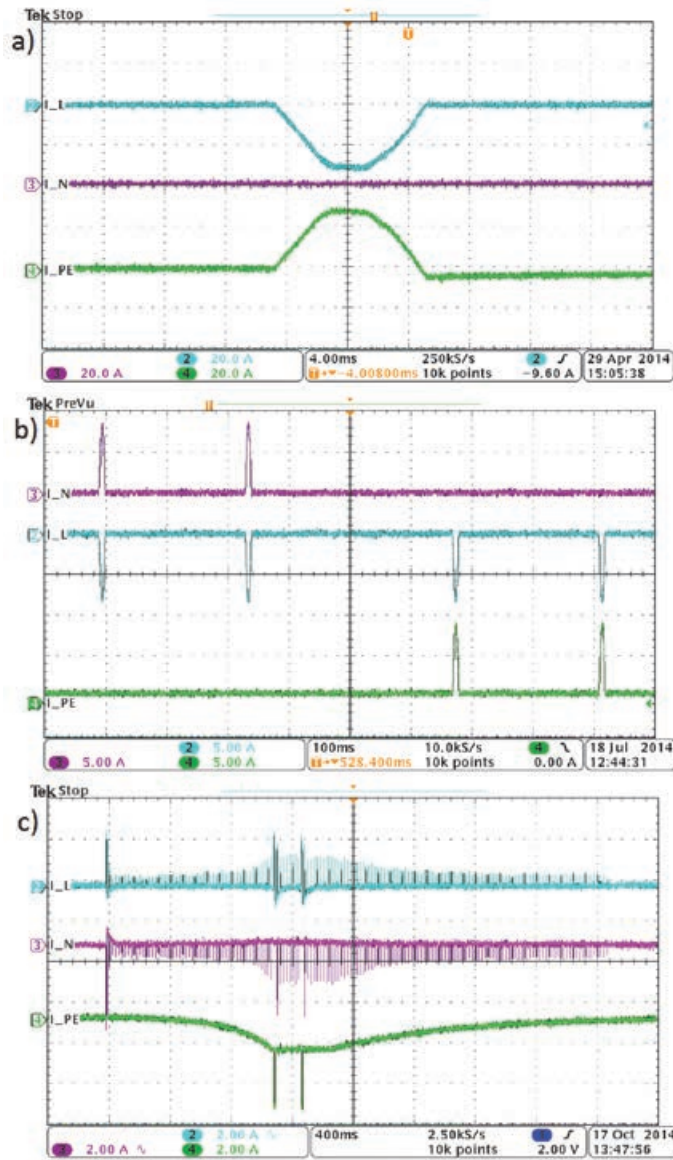
Fig. 4. Current waveforms in L, N and PE conductors during measurement without active ATT/RCD function, a) Sonel MPI-520 (scale 20 A/unit), b) Kyoritsu KEW 4140 (scale 5 A/unit), c) Kyoritsu 4120A 1 (scale 2 A/unit)
