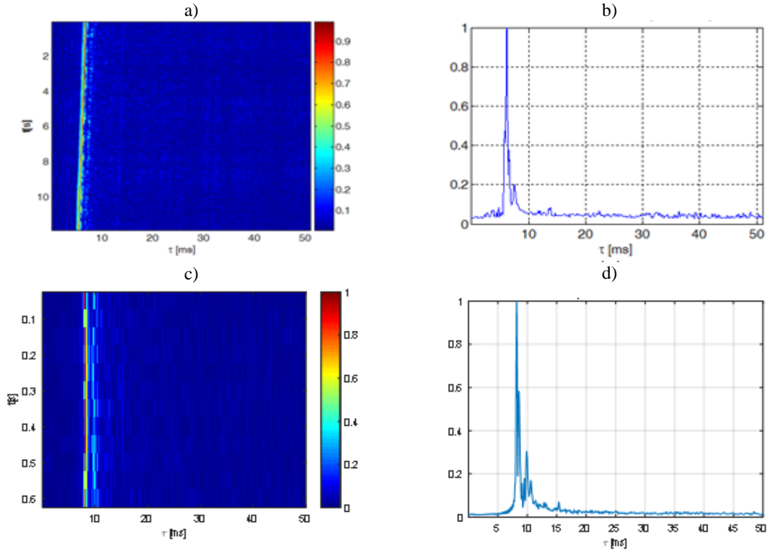
Fig. 6. Results of measurement at a distance of 550 m in bandwidth of 5kHz: module of CIR measured with PRBS (a) and its average over t-axis (b); module of CIR measured with HFM (c) and its average over t-axis (d).
