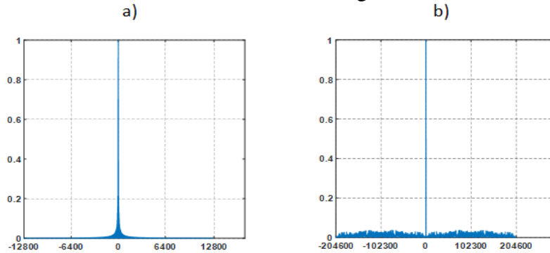
Fig. 1. Autocorrelation function of HFM (a) and PRBS (b) training signals.
