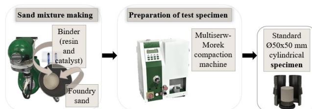
Fig. 2. Preparation of test specimens
