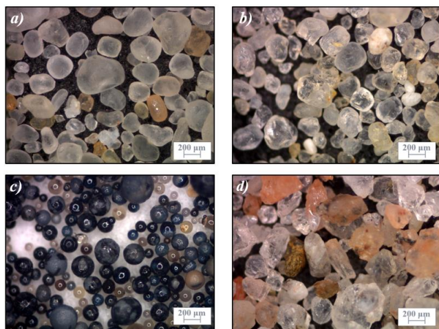
Fig. 1. Stereo microscopic images of the sands a) GBM 45, b) SH 33, c) Bauxite sand W55 and d) J-SAND at 20x magnification
