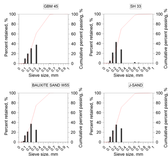
Fig. 5. Grain size distribution diagrams of the investigated sands
