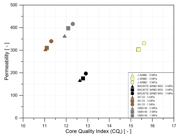
Fig. 7. The permeability test results as a function of CQ_i in the case of the investigated sands
