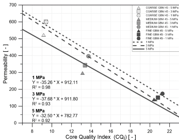
Fig. 6. The permeability test results as a function of CQ_i in the case of the fractionated GBM 45 quartz sand
