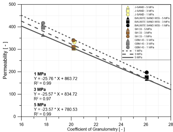
Fig. 8. The permeability test results as a function of CG in the case of the investigated sands
