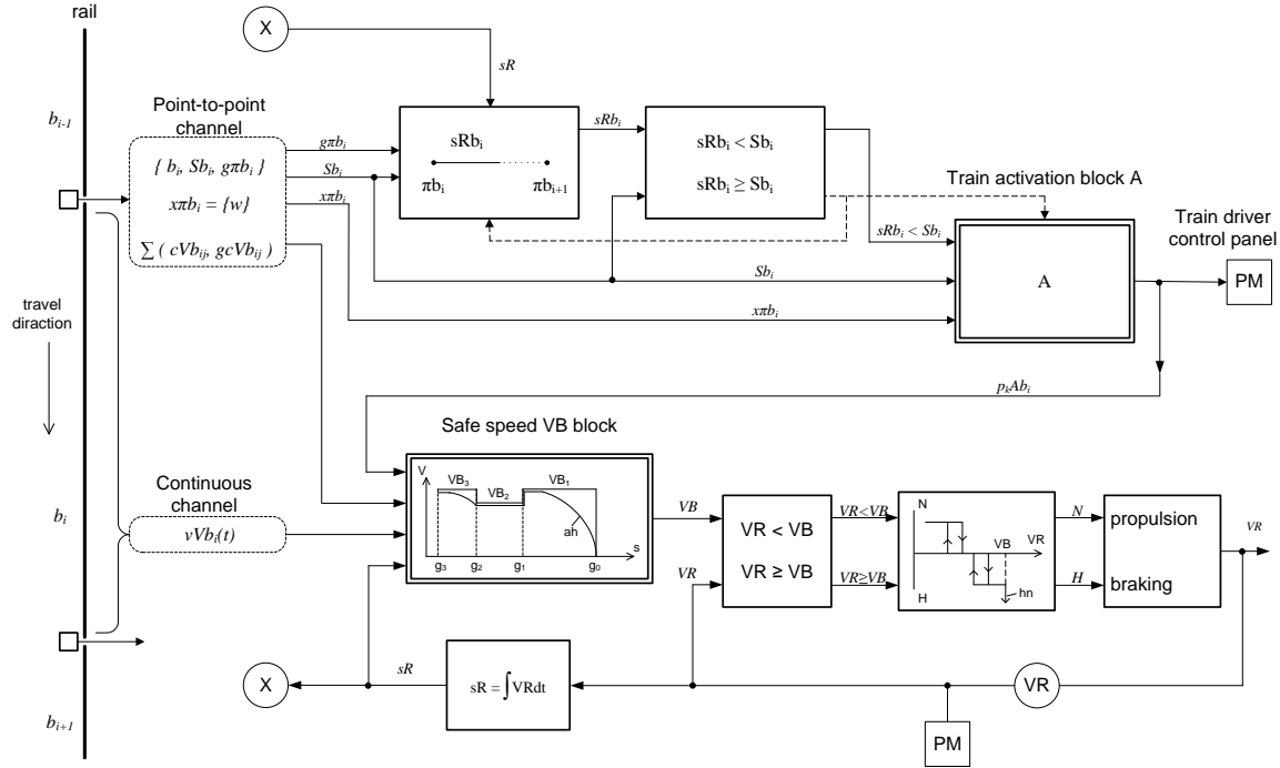
Fig. 10. Block diagram of ATP system, on-board option of determining systems VB .
