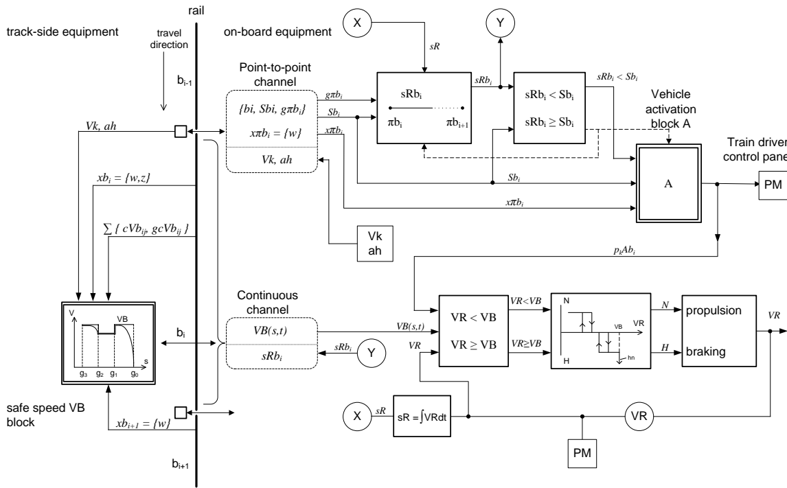
Fig. 11. Functional diagram of ATP system. The track-side option
