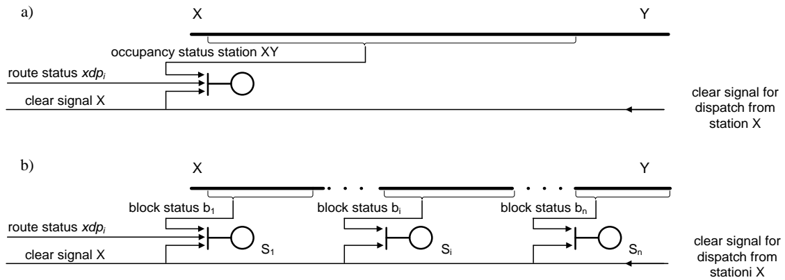
Fig. 4. Diagram showing safety procedure applying to wrong-way driving
