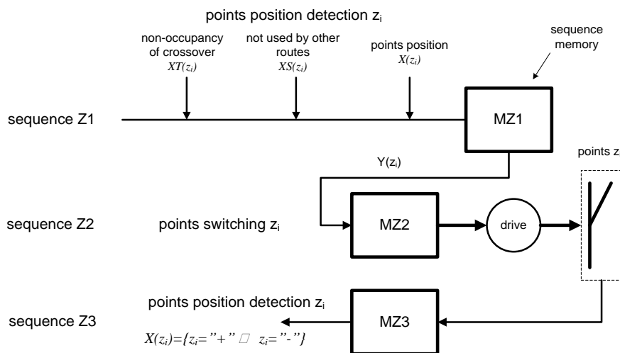
Fig. 1. Points switching sequences
