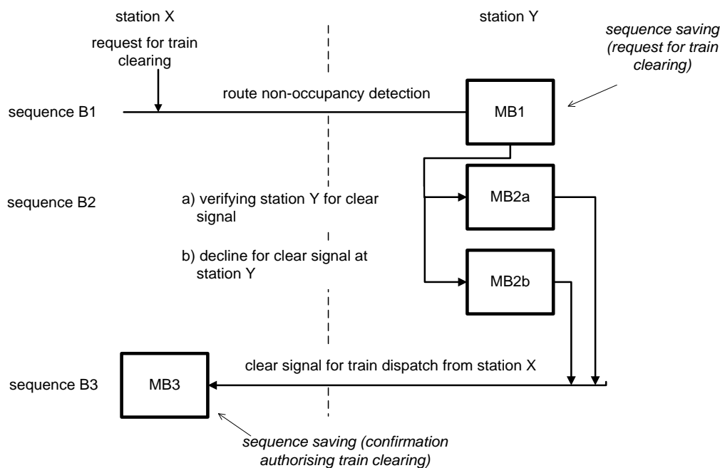
Fig. 3. The sequences line block operates to determine traffic direction
