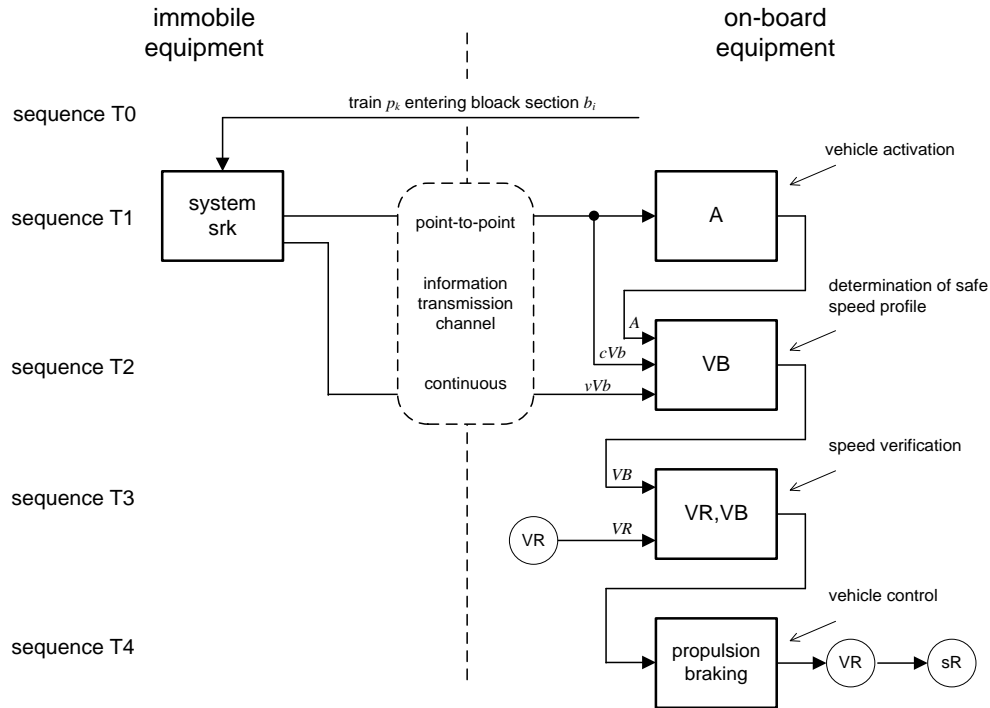
Fig. 7. ATP system operation upon entering next block section
