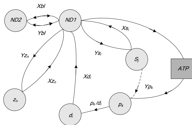
Fig. 5. Information flow in the process of controlling train traffic including the ATP system.
