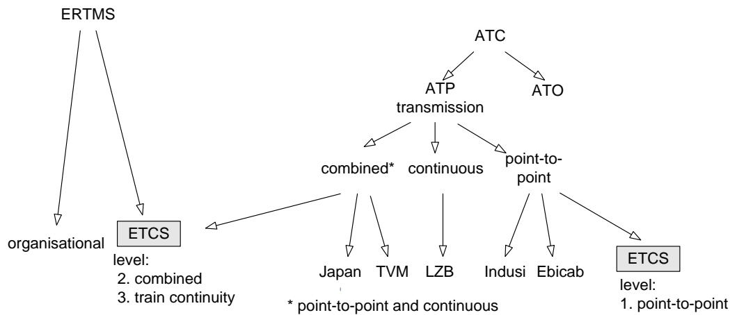
Fig. 15. ATP systems within ERTMS and ATC systems
