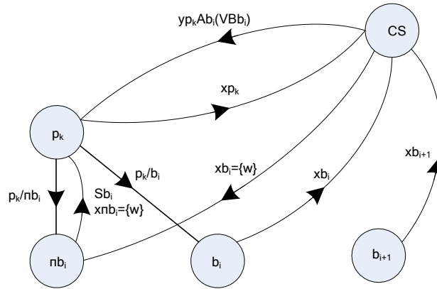
Fig. 6. Information flow graph for train control process
