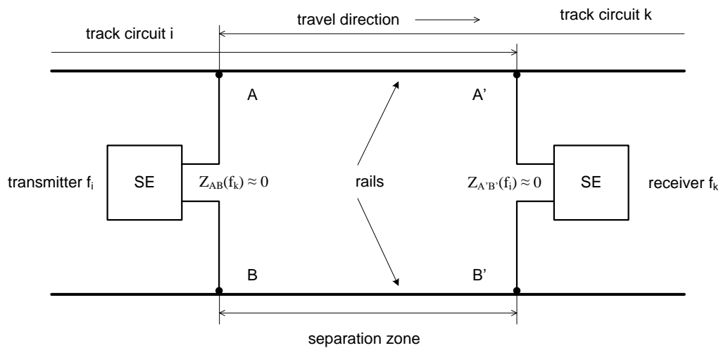
SE - electrical separation f_i, f_k – signal frequencies generated by transmitter and receiver of track circuits i and k
