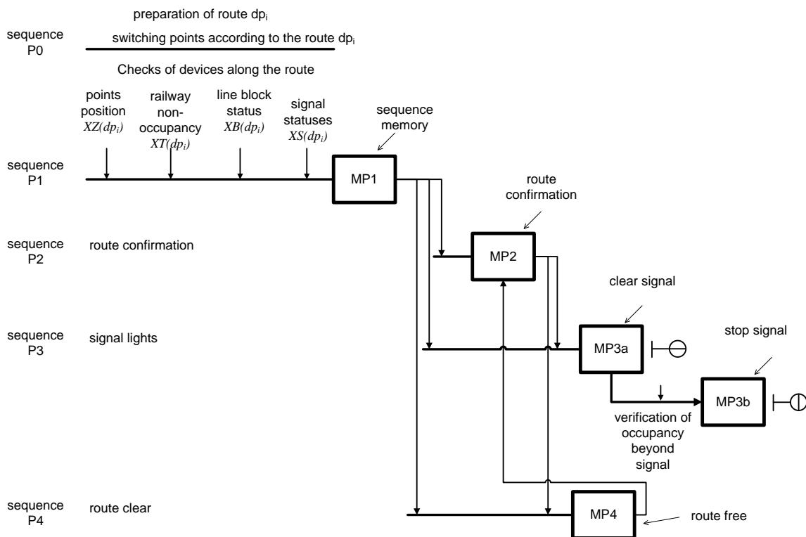
Fig. 2. Routing and signal light sequences
