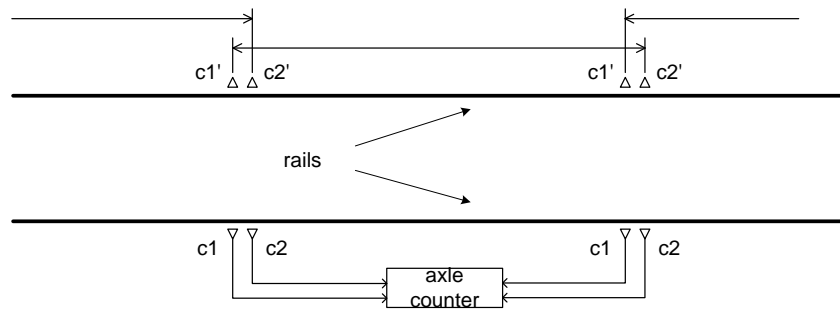
Fig. 14 Arrangement of sensors detecting axes at controlled track section
