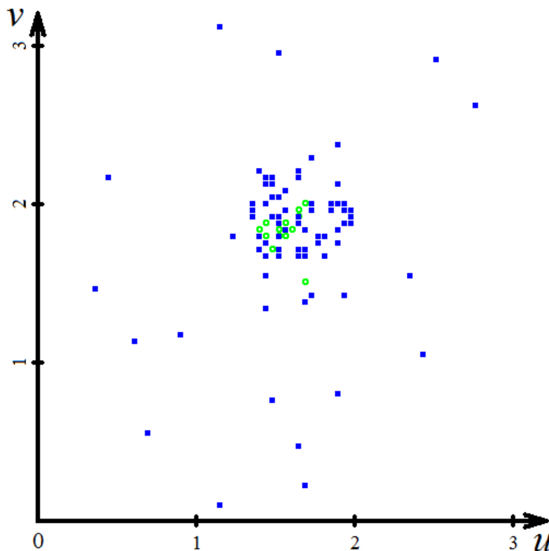
Fig. 2. View of 7-dimensional data representing coal samples of various suitability for fluidal gasification process by value of the parameter ITER = 5. The start of grouping is visible. The images of points representing coal samples less suitable for fluidal gasification process were marked as (■), images of points representing coal samples more suitable for fluidal gasification process were marked as (o)
