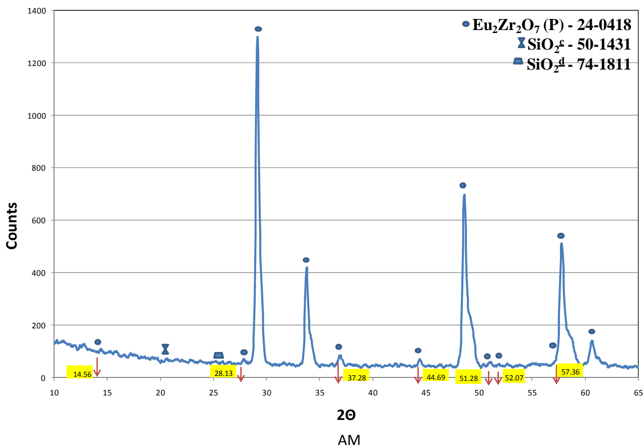
Fig. 6a. XRD diffraction patterns of sintered materials of \text{ZrO}_2 - \text{Eu}_2\text{O}_3 type after annealing process at temperature 1450^\circ\text{C} after DM and MA processes (HTPSA)
