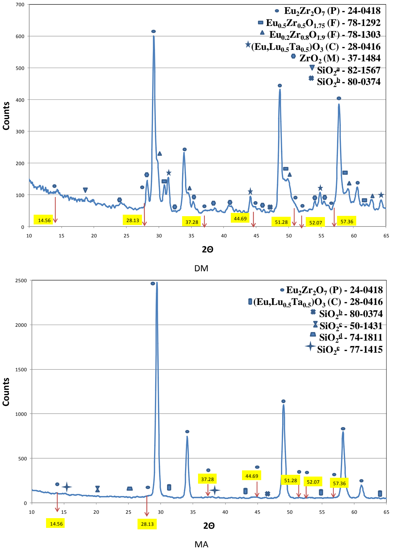
Fig. 4a. XRD diffraction patterns of sintered materials of ZrO 2 -Eu 2 O 3 type after DM and MA processes (HTPS)
