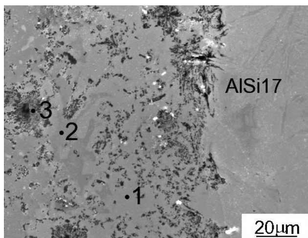
Fig. 6. Microstructure of the bonding zone close to the AlSi17 with points of the EDS quantitative analysis
