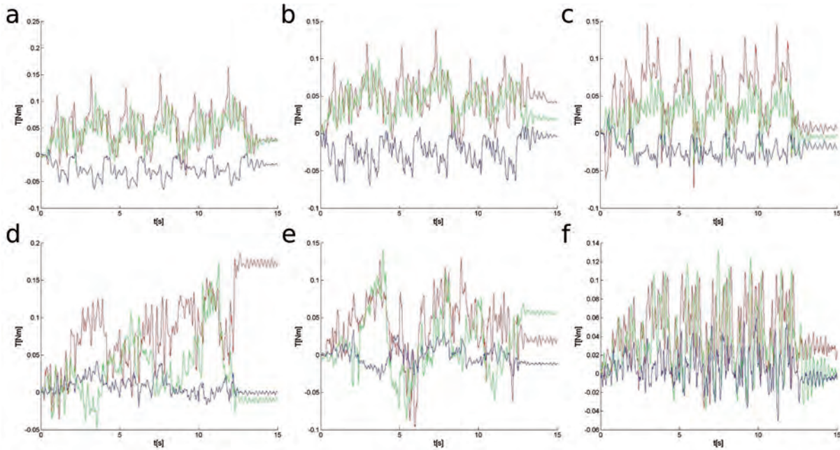
Fig. 5. Components of the contact torque vector for the robot walking on: soft ground (a), artificial grass (b), solid ground (c), gravel (d), pebbles (e), sand (f). Each component is marked with a color: red - T_x , green - T_y , blue - T_z
