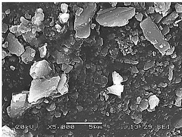
Fig. 1. SEM image of the waste marble powder (WMP)
