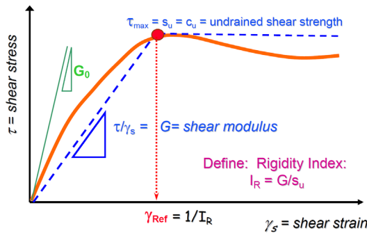
Figure 35: Shear stress vs. shear strain for soils and definition of t_{max} , G , g_s and I_R (after Mayne 2006).
