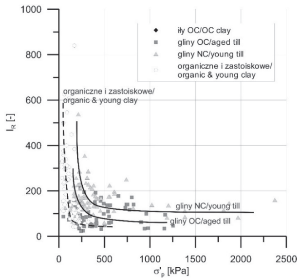
Figure 47: Rigidity index ( I_R ) vs. preconsolidation stress ( \sigma'_p ) (after Mlynarek et al. 2018).
