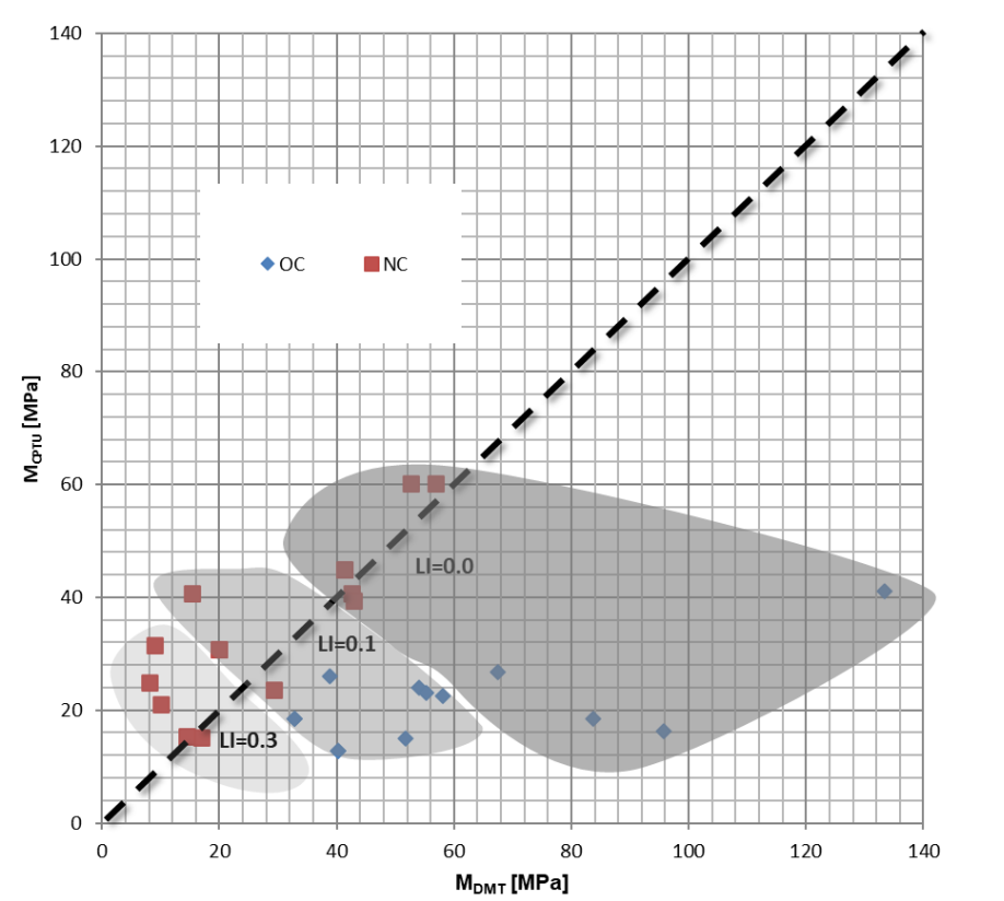
Figure 29: Comparison of M_{CPTU} and M_{DMT} values with M_{oeo} modulus (after Młynarek et al. 2016).
