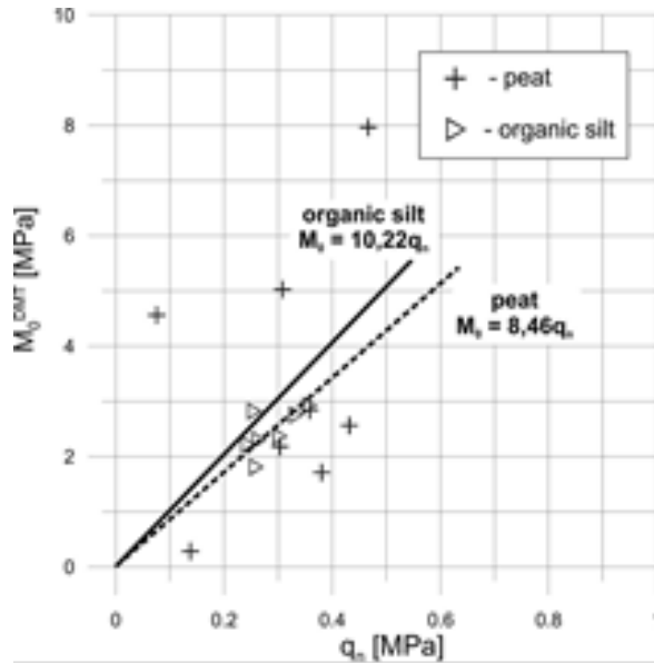
Figure 34: Correlation between constrained moduli M_o from DMT and q_n value from CPTU Młynarek et al. 2015.
