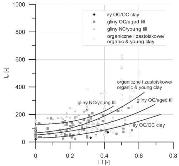
Figure 46: Rigidity index ( I_R ) vs. liquidity index ( LI ) (after Mlynarek et al. 2018).
