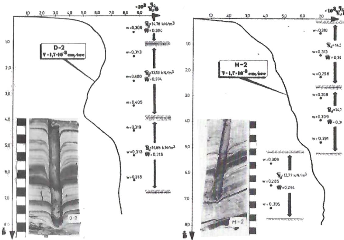
Figure 12 Static penetration diagram for horizontal (a) and diagonal (b) lamination of clay (after Młynarek et al. 1988), where: z —depth of penetration, D —cone diameter, \gamma_d —soil dry unit weight.
