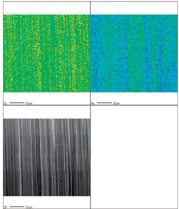
Fig. 11. Maps of element distribution (WDS) in Cu-Ag alloy. Section lengthwise to extrusion direction, magn. 2000x
