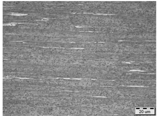
Fig. 6. Microstructure of Cu-Ag-Mm wire of diameter 6,4 mm, longitudinal section
