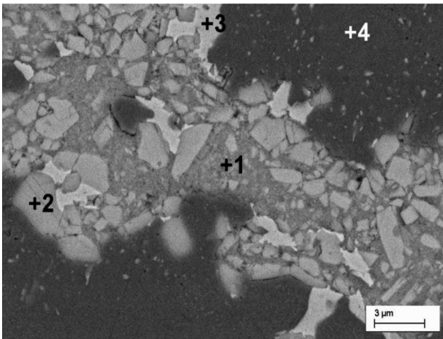
Fig. 4. Microstructure of Cu-Ag-Mm alloy with results of EDS microanalysis in microsections: 1: O=29.18%, La=25.13%, Ce=42.32%, Cu=3.37%; 2: O=34.72%, La=22.29%, Ce=40.26%, Cu=2.74%; 3: Ag=94.98%, Cu=5.02%; 4: Ag=4.97%, Cu=95.03%; polished section, SEM
