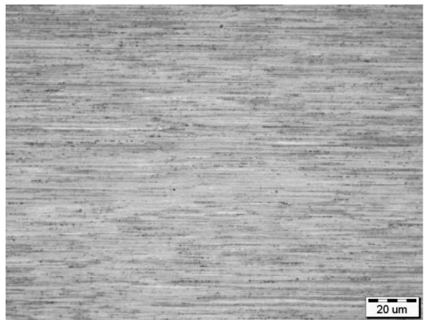
Fig. 7. Microstructure of Cu-Ag wire of diameter 0,50 mm, longitudinal section
