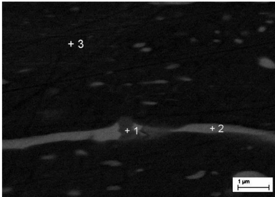
Fig. 10. Microstructure of Cu-Ag-Mm wire with results of EDS microanalysis in microsections: 1: Cu 50,3%, Ag 31,9%, O 11,0%, Ce 4,7%, La 2,1%; 2: Cu 24,5%, Ag 73,% 3: Cu 93,5%, Ag 6,5%; longitudinal section
