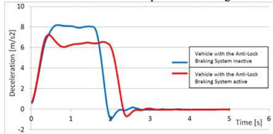
Fig. 8. Diagram presenting the braking deceleration differences in the case of the vehicle with shock absorbers in good working condition on the N2 surface
