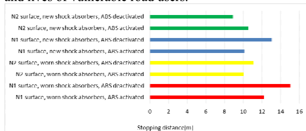
Fig. 9. Diagram showing the changes of stopping distance with three parameters taken into consideration
