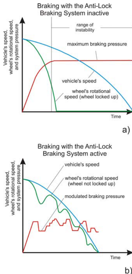
Fig. 1. Changes of the braking parameters a) without the Anti-Lock Braking System and b) with the Anti-Lock Braking System [authors' own elaboration on the basis of 12]
