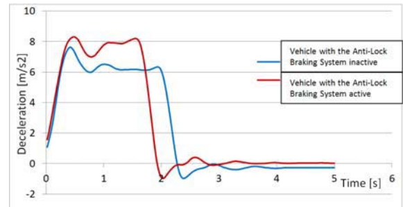
Fig. 6. Diagrams presenting the braking deceleration differences in the case of the vehicle with worn shock absorbers on the N2 surface.
