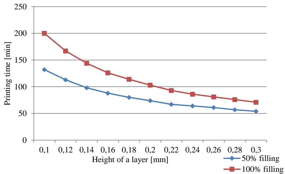
Figure 6. Relation of printing time to the layer height of the model (author's own study)
