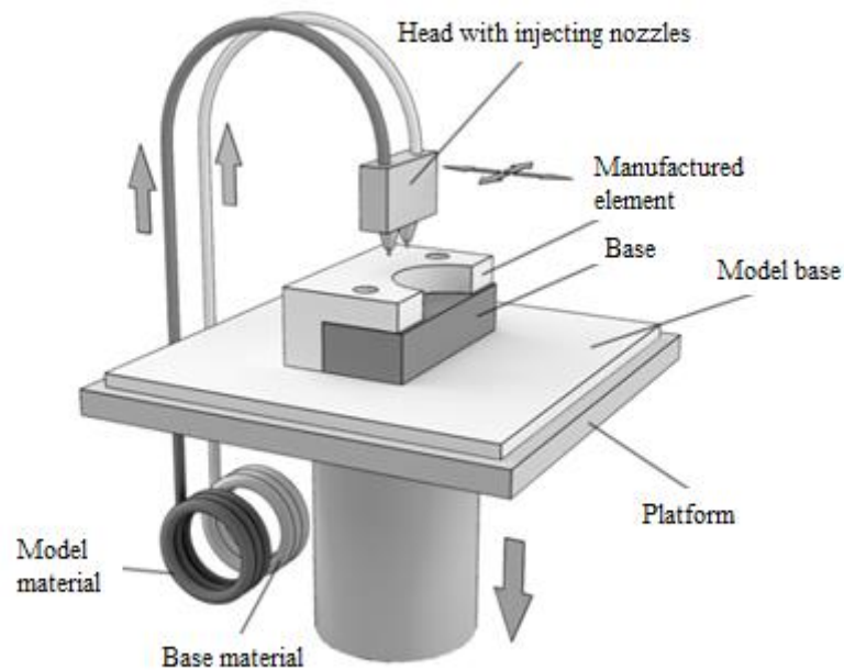
Figure 1. Principle of FDM technology performance (Kiński and Pietkiewicz, 2018)
