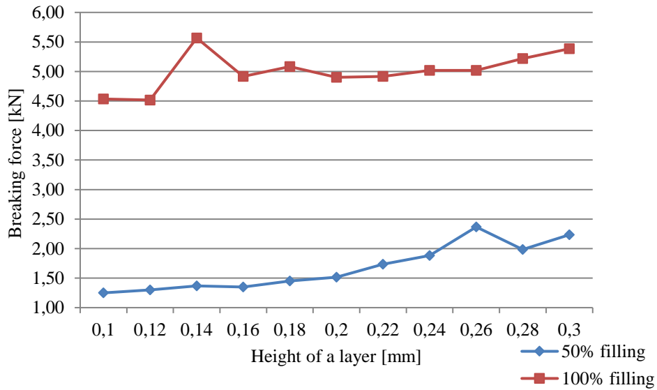
Figure 5. Average force that breaks a sample in relation to the height of the print layer (author's own study)
