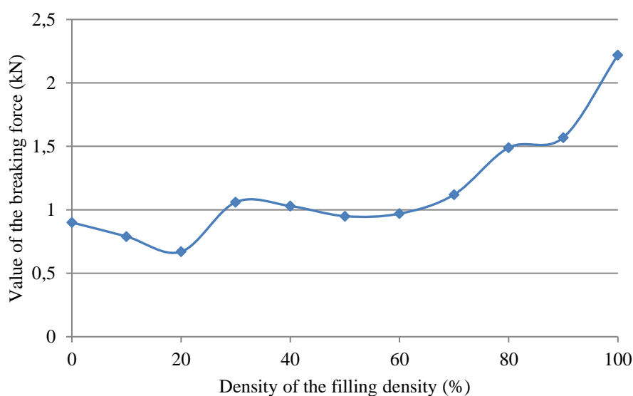
Figure 3. Results of research on the relation of the breaking force to the filling (Miazio, 2015)
