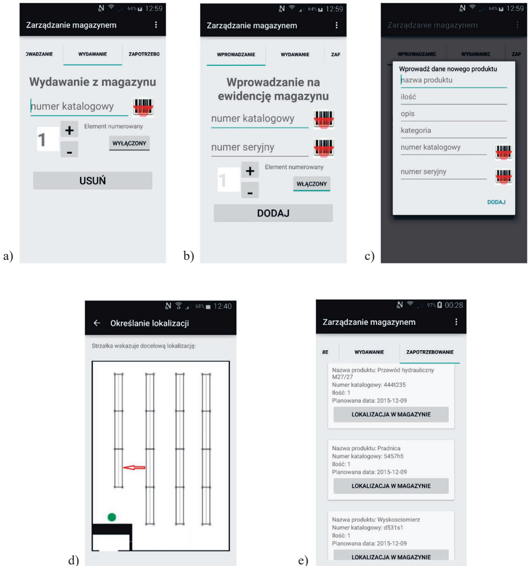
Fig. 7. Screenshots showing functions of the warehouseman’s profile: a) issuing from the warehouse; b) entering to the inventory; c) defining a new product; d) specifying its location; e) checking demand [Kawka, 2016]
