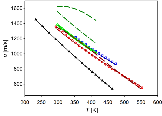
Fig. 2. Speeds of sound in saturated alkanes. Points – experimental data: circles – n -octane (NERUCHEV et al. , 2005), downward triangles – n -hexadecane (NERUCHEV et al. , 2005), crossed circles – n -tetracosane (NERUCHEV et al. , 2005), upward triangles – squalene (KOROTKOVSKII et al. , 2012); solid lines – predictions of the proposed approach; dashed lines – predictions of the previous method (POSTNIKOV, 2016) for n -hexadecane and squalene; dash-dotted line – prediction of the described approach without the boiling point correction for squalene.
