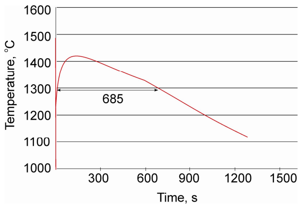
Fig. 6. The curve of temperature changes in time; thermocouple pad; cubicoid 80x80x100mm (pouring temperature 1510°C)
