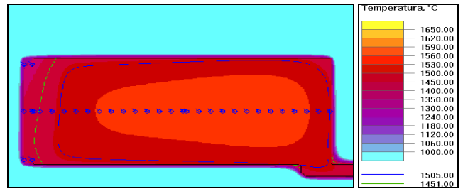
Fig. 7. Temperature distribution after 45 s; cubicoid 70x70x150[mm]; pouring temperature 1600°C
