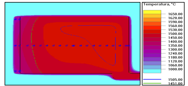
Fig. 9. Temperature distribution after 45 s; cubicoid 80x80x100[mm]; pouring temperature 1510°C
