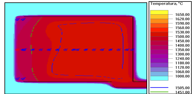
Fig. 8. Temperature distribution after 45 s; cubicoid 90x90x80[mm]; pouring temperature 1550°C
