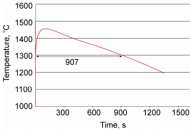
Fig. 4. The curve of temperature changes in time; thermocouple pad; cubicoid 70x70x150mm (pouring temperature 1600°C)
