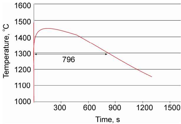
Fig. 5. The curve of temperature changes in time; thermocouple pad; cubicoid 90x90x80mm (pouring temperature 1550°C)
