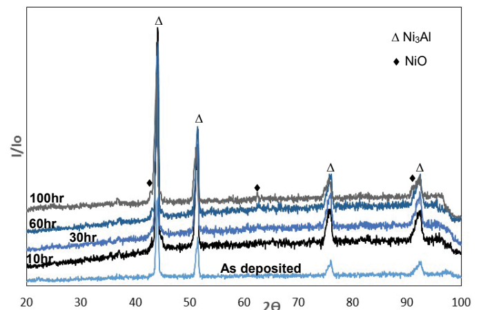
Fig. 8. Comparison of XRD results of Ni 3 Al coating treated at 500°C for different times
