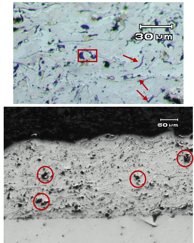
Fig. 2. As sprayed Nickel Aluminide coating showing different features of the coating i.e. porosity (encircled), oxide layers (arrows) and unmelted particles (dotted box)
