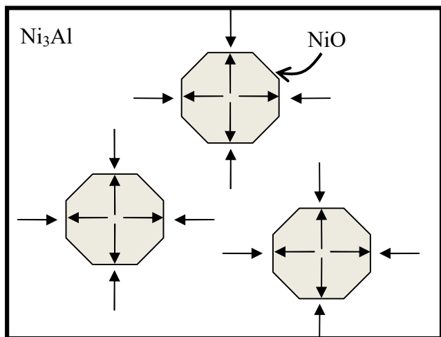
Fig. 14. Schematic demonstrates that NiO phase exerted tensile stresses due to which the matrix (Ni 3 Al) becomes in compressive stress
