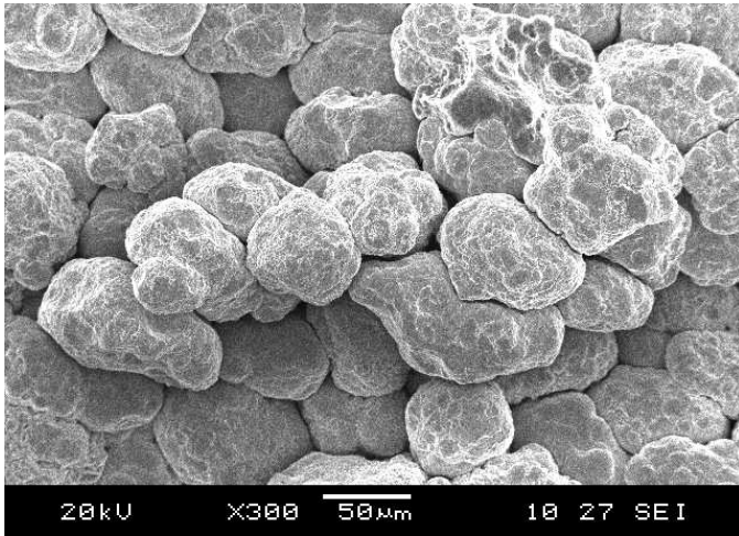
Fig. 1. SEM image showing the morphology of spraying powder
