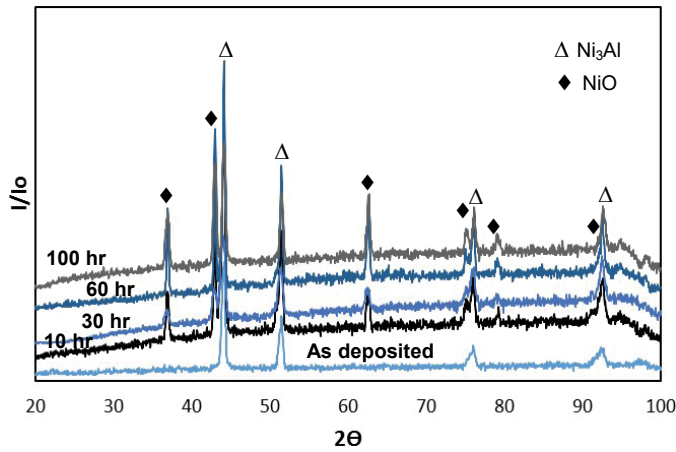
Fig. 11. Comparison of XRD results of Ni 3 Al coating treated at 800°C for different times
