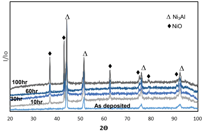
Fig. 10. Comparison of XRD results of Ni 3 Al coating treated at 700°C for different times
