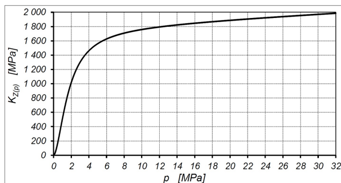
Fig. 7. Bulk modulus K_{Z(p)} of Total Azolla ZS 46 mineral oil [36, 37, 55]
