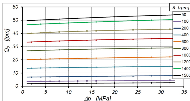
Fig. 8. Flow rate Q_2 vs \Delta p at n = const
